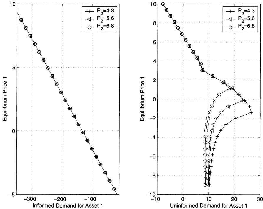
Figure 8. Price and investor demand for asset 1. The lines with +, with \Delta , with \circ in the left (right) graph represent informed (uninformed) investor demand for asset 1 as a function of asset 1 price when asset 2 price is 4.3, 5.6, and 6.8, respectively. The informed investor demand schedules in the left graph are drawn when the realized signal shocks in Markets 1 and 2 are both -6 .
