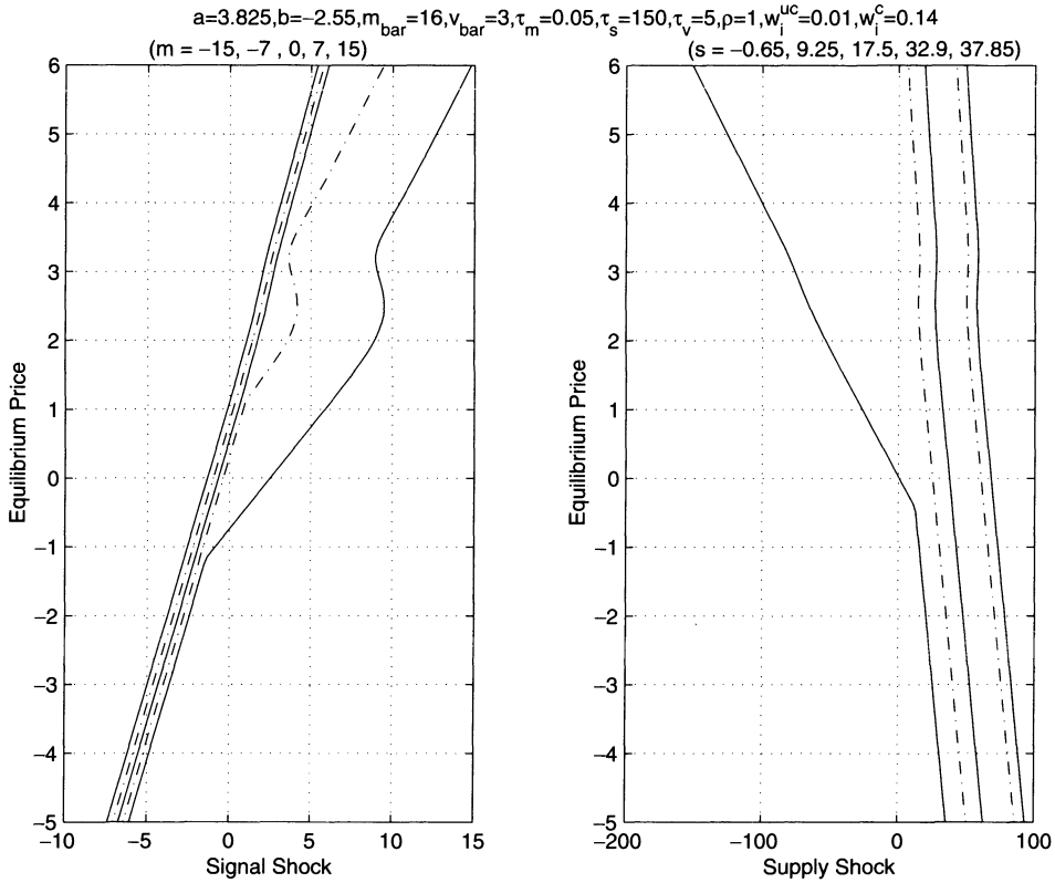
Figure 5. Price sensitivity to signal and supply shocks. The lines in the left graph represent equilibrium price as a function of the signal shock when the supply shock is -15, -7, 0, 7 , and 15 , respectively. The lines in the right graph represent equilibrium price as a function of the supply shock when the signal shock is -0.65, 9.25, 17.5, 32.9 , and 37.85 , respectively.
