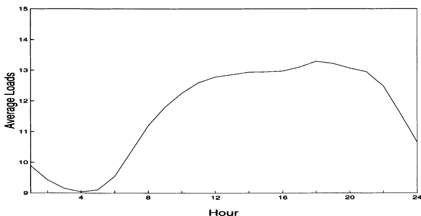
Figure 3. Average electricity demand. This figure plots the average load in gigawatt hours for each of the 24 hours.
