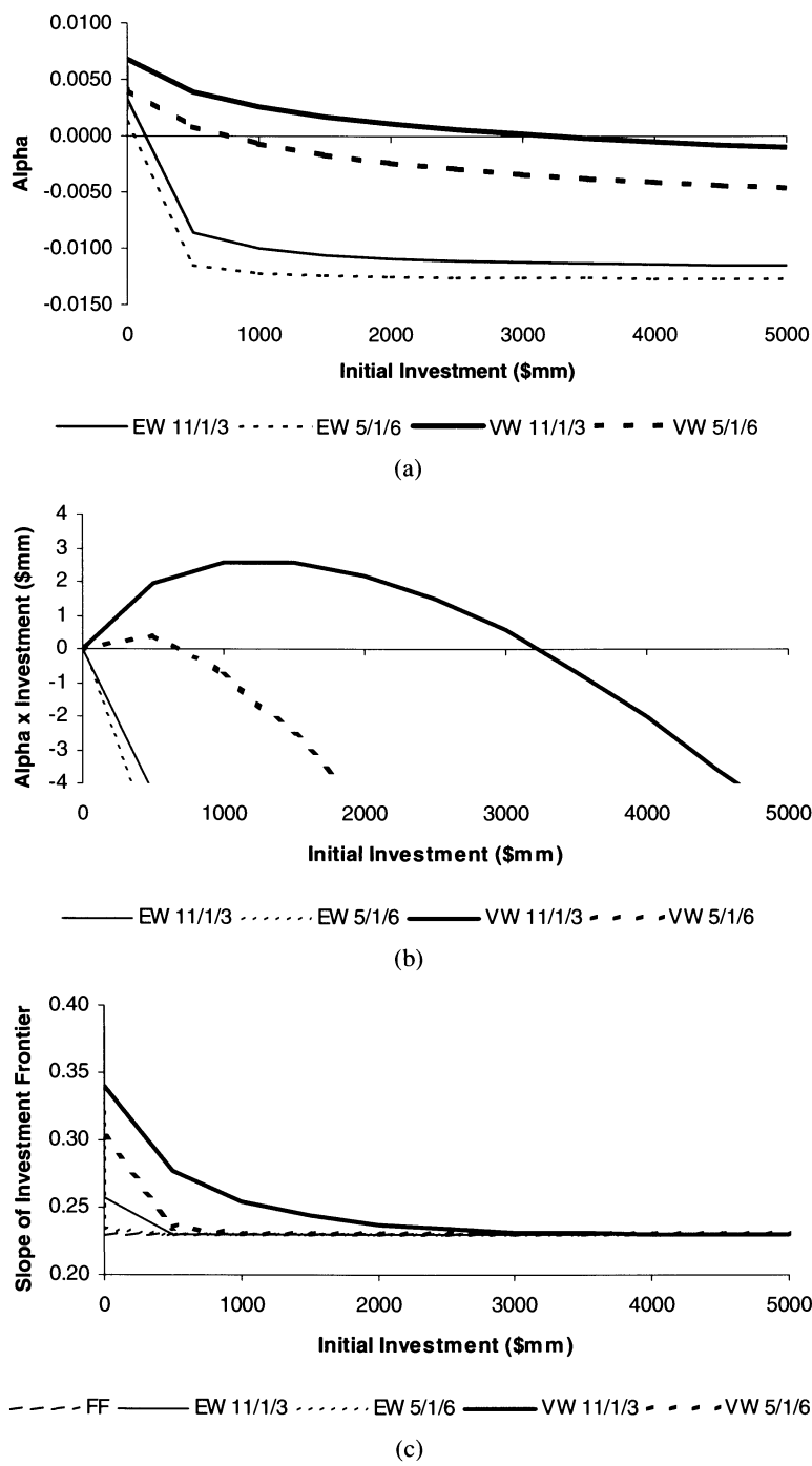
Figure 6. Performance evaluation of momentum strategies (NYSE, AMEX, and Nasdaq, Breen-Hodrick-Korajczyk). We evaluate the performance of momentum trading strategies
