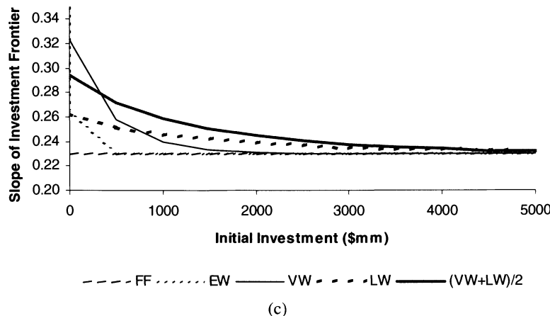
Figure 4. Performance evaluation of momentum strategies (NYSE, Breen-Hodrick-Korajczyk). We evaluate the performance of momentum trading strategies using the trading
