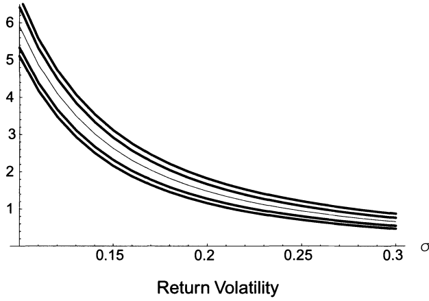
Figure 10. Boundaries as functions of the return volatility. The graph plots the optimal boundaries \bar{z} , z^* , \bar{z}^* , and \bar{z} against return volatility \sigma for the following parameters: time discount rate \delta = 0.01 , risk-free rate r = 0.01 , expected return \mu = 0.069 , proportional cost \alpha = 0.01 , fixed cost F = 5 , and absolute risk aversion coefficient \beta = 0.001 .
