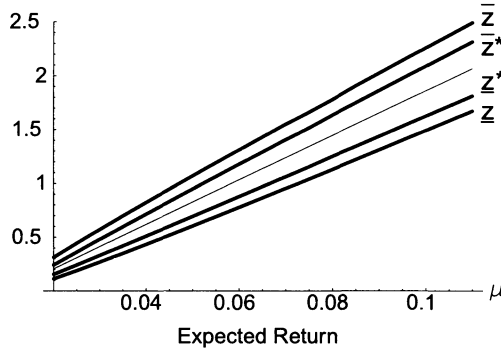
Figure 11. Boundaries as functions of the expected return. The graph plots the optimal boundaries \bar{z} , z^* , \bar{z}^* , and \bar{z} against expected return \mu for the following parameters: time discount rate \delta = 0.01 , risk-free rate r = 0.01 , return volatility \sigma = 0.22 , proportional cost \alpha = 0.01 , fixed cost F = 5 , and absolute risk aversion coefficient \beta = 0.001 .
