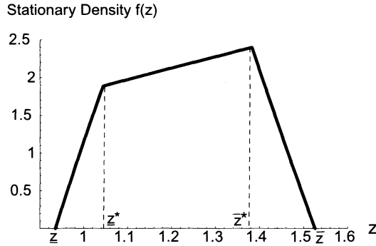
Figure 16. The stationary density function of the amount in a stock. The graph plots the stationary density function f(z) for the following parameters: time discount rate \delta = 0.01 , risk-free rate r = 0.01 , expected return \mu = 0.069 , return volatility \sigma = 0.22 , proportional cost \alpha = 0.01 , fixed cost F = 5 , and absolute risk aversion coefficient \beta = 0.001 .
