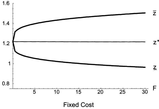
Figure 2. Boundaries as functions of the fixed cost. The graph plots the optimal boundaries \bar{z} , z^* , and \underline{z} against fixed cost F for the following parameters: time discount rate \delta = 0.01 , risk-free rate r = 0.01 , expected return \mu = 0.069 , return volatility \sigma = 0.22 , proportional cost \alpha = 0 , and absolute risk aversion coefficient \beta = 0.001 .
