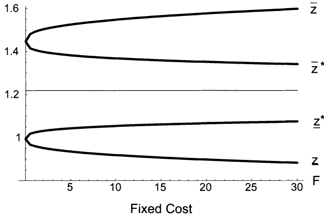
Figure 6. Boundaries as functions of the fixed cost. The graph plots the boundaries \bar{z} , \bar{z}^* , z^* , and z against fixed cost F for the following parameters: time discount rate \delta = 0.01 , risk-free rate r = 0.01 , expected return \mu = 0.069 , return volatility \sigma = 0.22 , proportional cost \alpha = 0 , and absolute risk aversion coefficient \beta = 0.001 . The thin middle line is the Merton line.
