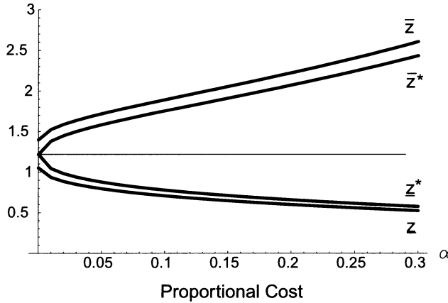
Figure 7. Boundaries as functions of the proportional cost. The graph plots the boundaries \bar{z} , z^* , \bar{z}^* , and \underline{z} against proportional cost \alpha for the following parameters: time discount rate \delta = 0.01 , risk-free rate r = 0.01 , expected return \mu = 0.069 , return volatility \sigma = 0.22 , fixed cost F = 5 , and absolute risk aversion coefficient \beta = 0.001 . The thin middle line is the Merton line.
