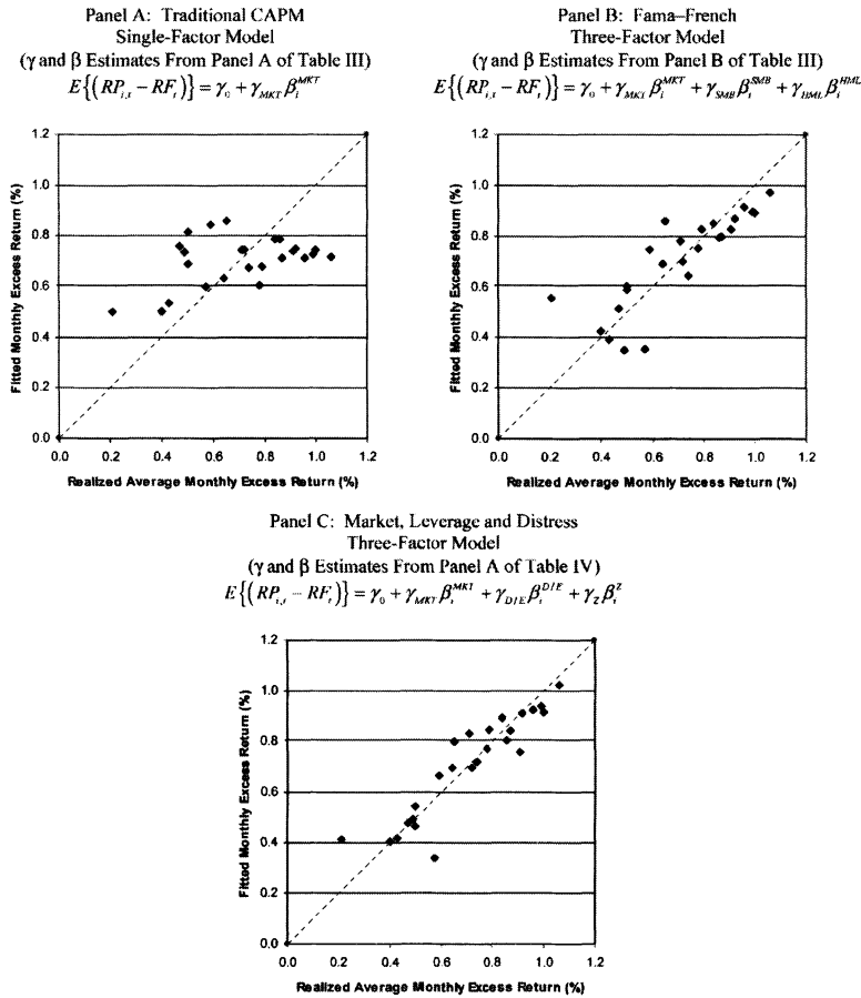
Figure 1. Plots of fitted versus actual returns for 25 Fama-French portfolios July 1964 – December 2000 (438 months). The three panels present plots of fitted-versus-actual average monthly returns for the cross-sectional models in Table III and Panel A of Table IV. In Panel A, \beta_i^{MKT} is the estimated slope coefficient from a time-series regression of (RP_{i,t} - RF_t) on a constant and (R_t^{MKT} - RF_t) . In Panel B, \beta_i^{MKT} , \beta_i^{SMB} , and \beta_i^{HML} are the estimated slope coefficients from a regression of (RP_{i,t} - RF_t) on a constant, (R_t^{MKT} - RF_t) , R_t^{SMB} , and R_t^{HML} where R_t^{SMB} is the return on the Fama-French small minus big portfolio in month t , and R_t^{HML} is the return on the Fama-French high minus low (book-to-market) portfolio in month t . In Panel C, \beta_i^{MKT} , \beta_i^{D/E} , and \beta_i^Z are the estimated slope coefficients from a regression of (RP_{i,t} - RF_t) on a constant, (R_t^{MKT} - RF_t) , R_t^{D/E} , and R_t^Z . In all three specifications, R_t^{MKT} is the value-weighted return on all stocks in the Fama-French 25 for month t , and RP_{i,t} is the return on the Fama-French size/book-to-market portfolio i ( i = 1, \dots, 25 ) in month t . In June of each year t , firms are assigned to one of three D/E portfolios based on NYSE breakpoints and (independently) one of two Z portfolios ( Z < 2.675 and Z > 2.675 ). The time series of leverage and distress portfolio returns R_t^{D/E} and R_t^Z are constructed each month by calculating the simple average return on the two high- D/E portfolios minus the simple average return on the two low- D/E portfolios (for R_t^{D/E} ) and the simple average return on the three high- Z portfolios minus the simple average return on the three low- Z portfolios (for R_t^Z ).
