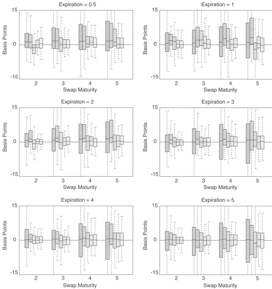
Figure 4. Box and whisker plots of swaption straddle gamma hedging errors. This figure presents the box and whisker plots for the one-week hedging errors, for swaption straddles across all expirations, and underlying swap maturities. The corresponding plots for the unhedged straddles are presented for comparison purposes. In each figure, the first box corresponds to the unhedged swaption, the second box to the one-factor model, the third box to the two-factor model, the fourth box to the three-factor model, and the fifth box to the four-factor model.
