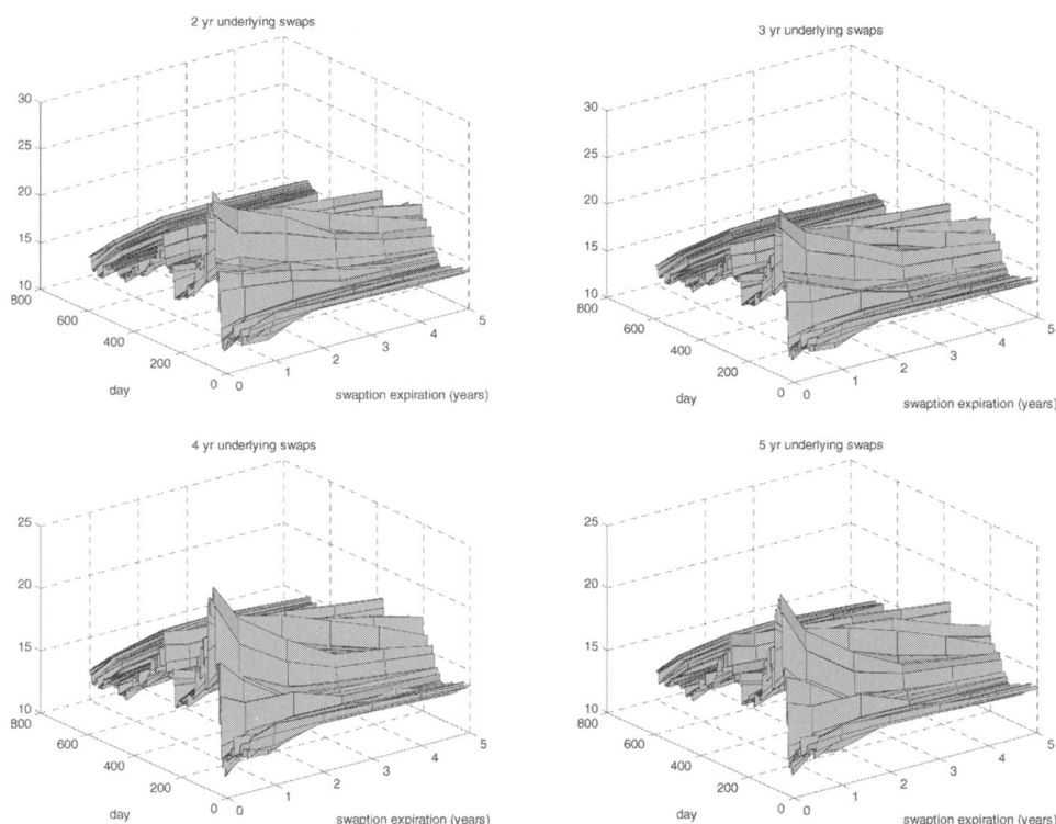
Figure 1. Time series of swaption volatilities. The figures present the time series of the swaption volatility term structures for each underlying swap maturity, over the data sample period, from March 1, 1998, to October 31, 2000. The volatilities shown are Black volatilities of the underlying forward swap rates.
