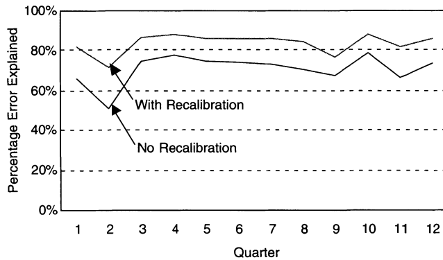
Figure 6. Time series of swaption straddle hedging errors explained by the four-factor model. The figure compares the time series of the percentage of straddle hedging errors explained by the four-factor model across all contracts by quarter, when the eigenvalues of the four-factor model are updated every second week, with the percentage from the same model with no parameter updating. In the figure, the lower line represents the percentage of the unhedged straddle error, as measured by the total sum of squared error for all contracts over the quarter, explained by the four-factor model with no recalibration. The upper line represents the corresponding percentage for the four-factor model when it is periodically recalibrated. Each percentage is based on 144 observations.
