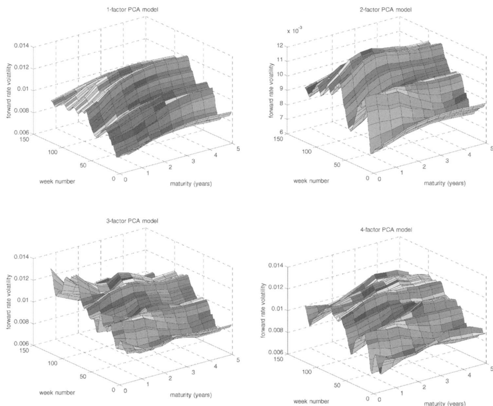
Figure 2. Estimated volatilities of forward rates implied from swaption prices. The figures present the time series of estimated forward rate volatilities for all the models. There are 70 volatility curves on each figure, with each curve separated by two weeks. The data for these curves are derived from the 70 optimization problems for each model.
