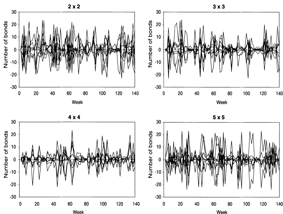
Figure 5. Time series of straddle delta-gamma hedge portfolios for the four-factor model. This figure presents the time series of the number of bonds in the delta-gamma hedge portfolios constructed for swaption straddles using the four-factor model. The hedge portfolio compositions are shown for four representative straddle contracts ( 2 \times 2 , 3 \times 3 , 4 \times 4 , and 5 \times 5 ) over a period of 140 weeks (March 1998 to October 2000). The hedge portfolio at each week consists of long or short positions in eight bonds, ranging from 1 year to 10 years in maturity.
