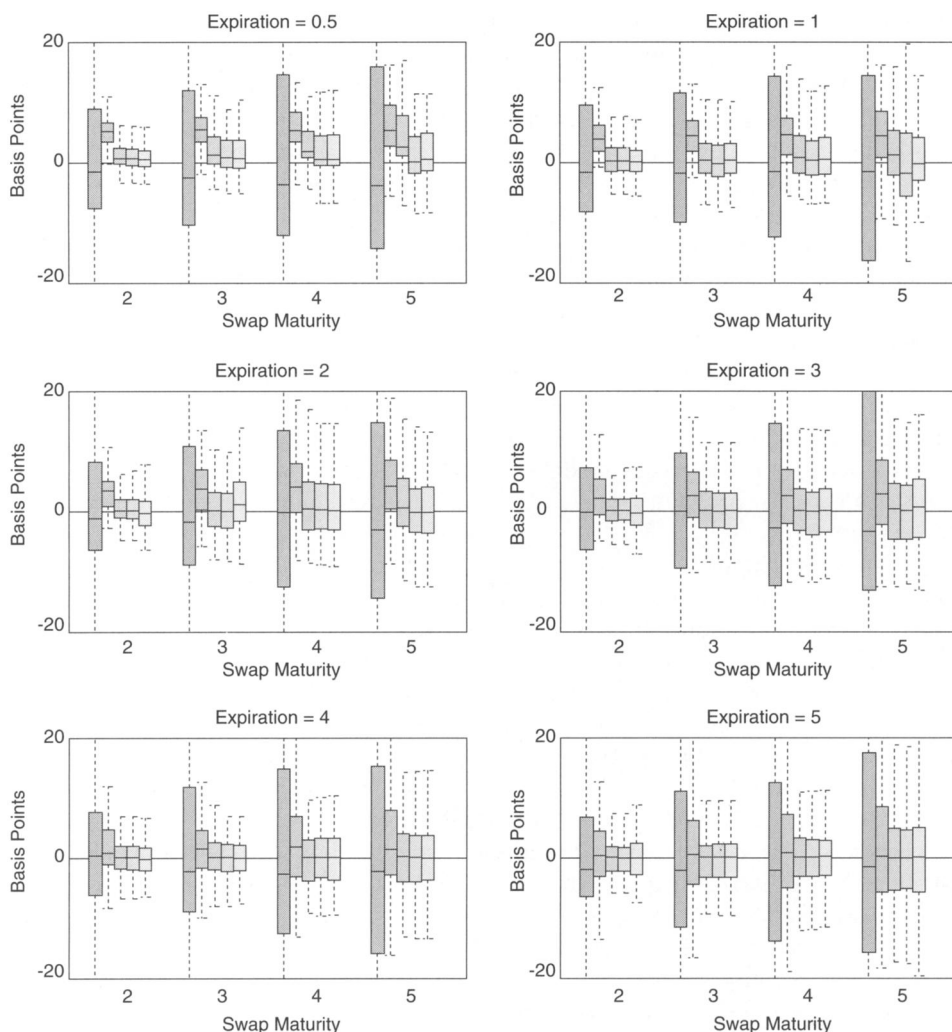
Figure 3. Box and whisker plots of swaption hedging errors. This figure presents the box and whisker plots for the one-week hedging errors, for swaptions across all expirations and underlying swap maturities. The corresponding plots for the unhedged swaptions are presented for comparison purposes. In each figure, the first box corresponds to the unhedged swaption, the second box to the one-factor model, the third box to the two-factor model, the fourth box to the three-factor model, and the fifth box to the four-factor model.
