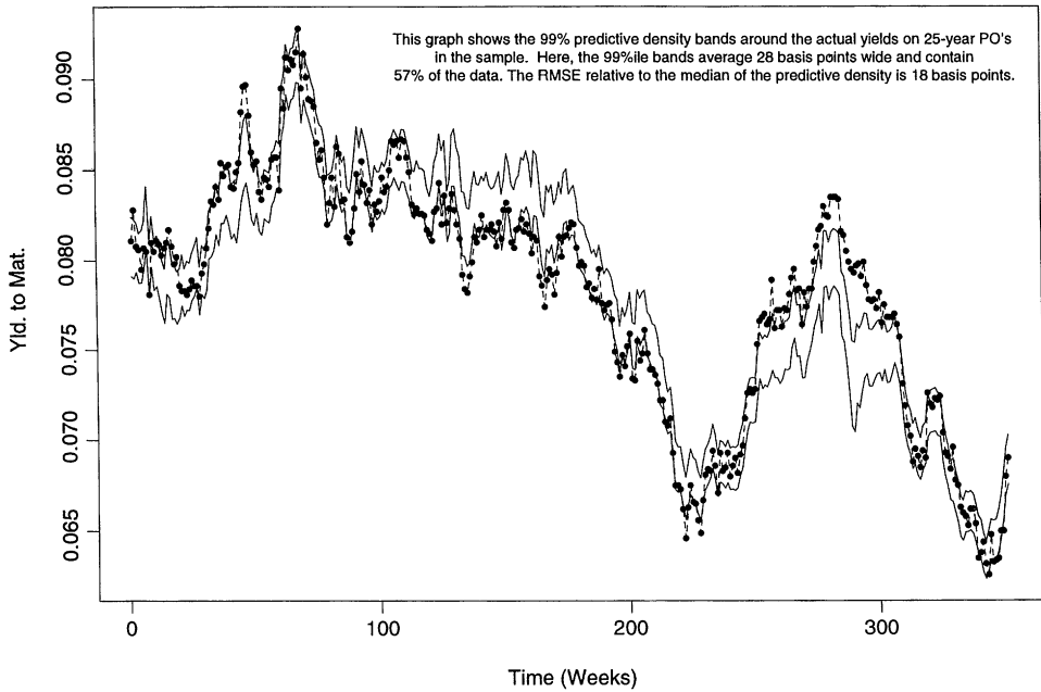
Figure 5. Time series of 25-year bond yield. Ninety-ninth percentile predictive density bands from the three-factor CIR model, overlaid the data, which are weekly observations of yields on 25-year principal only strips of U.S. Treasury bonds.
