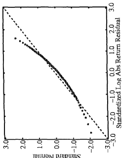
QQ Plot
