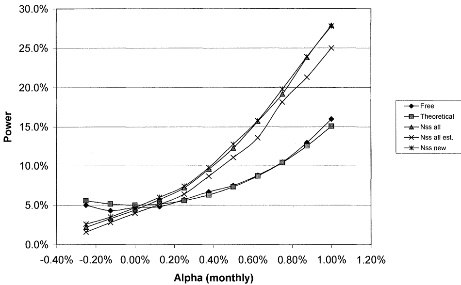
Figure 1. Power functions. The figure presents the power function as a function of the intercept in equation (19a). For each value of the intercept (Alpha), the power is derived from a series of 1,000 simulations with 120 monthly observations each, when the rejection rate is 5 percent. The theoretical power is presented (Theoretical) as well as the power for the test with no short sales constraints (Free), with short sales constraints on the new asset only (Nss new) and with short sales constraints on all assets (Nss all) in case the benchmark assets are known, and with short sales constraints on the new assets when the benchmark assets are estimated during the simulations (Nss all est.).
