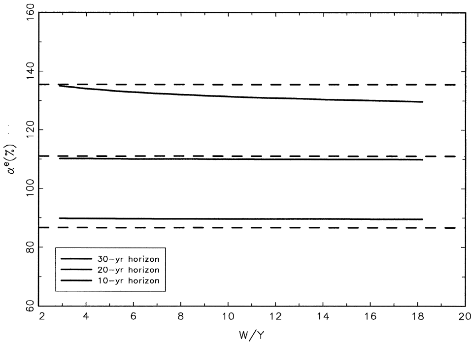
Figure 4. Optimal portfolio allocation to stocks in the employment state: Numerical and approximate analytical solutions. The graph plots the numerical and the approximate analytical solution for the optimal portfolio allocation to stocks against the financial wealth–labor income ratio. The dashed horizontal lines within the graph correspond to the approximate analytical solution, and the solid lines to the numerical solution. The graph plots the solutions for three expected retirement horizons: 30 years (top lines), 20 years (middle lines) and 10 years (bottom lines). These solutions assume the following parameter values: \gamma = 3 , \delta = 1/(1.10) , E_t[Y_{t+1}/Y_t] = \exp\{g + \sigma_\xi^2/2\} = 1.03 , \sigma_\xi = 0.10 , R_f = 1.02 , E_t[R_{1,t+1}/R_f] = \exp\{\mu + \sigma_u^2/2\} = 1.06 , and \sigma_u = 0.18 . The expected lifetime after retirement is 10 years. All covariances are set to zero.
