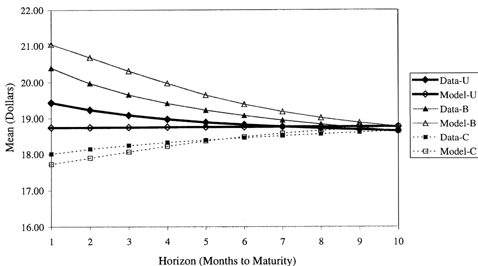
A: Mean Normalized Forward Price
