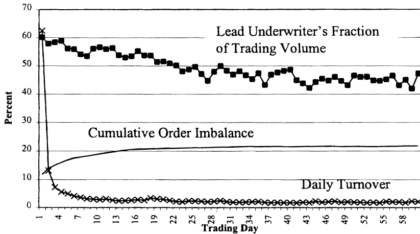
Figure 1. Mean daily turnover, cumulative order imbalance, and the lead underwriter's fraction of trading. The average daily turnover is shown for the sample of 306 IPOs. Average daily turnover is measured as the number of shares traded as a fraction of the number of shares offered in the IPO (not including overallotment shares). The cumulative order imbalance is the cumulative sell-initiated volume minus the cumulative buy-initiated volume, as a fraction of the shares offered in the IPO. Buy/sell direction is given directly in the NASD transactions data for 80 percent of the trades, and the Lee and Ready (1991) algorithm is used for the remaining 20 percent. The lead underwriter's trading volume is the number of shares traded by the lead underwriter as a liquidity provider, as a fraction of the total daily trading volume. The lead underwriter is a liquidity provider in a trade when he sells (buys) in a buyer (seller) initiated trade.
