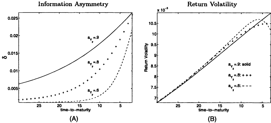
Figure 6. Time-to-maturity patterns of information asymmetry and futures return volatility for various values of \alpha_{Y_2} —persistence of nonmarketed risk shocks. The figures plot the time-to-maturity patterns of (A) information asymmetry, \delta , and (B) the return volatility of the k th contract. The parameters are set at the following values: \kappa_{Dq} = 0.5 , \sigma_D = 0.2 , \sigma_q = 0.025 , a_Z = 0.98 , \sigma_Z = 0.025 , a_{Y_1} = 0.97 , \sigma_{Y_1} = 0.075 , \sigma_{Y_2} = 0.05 .
