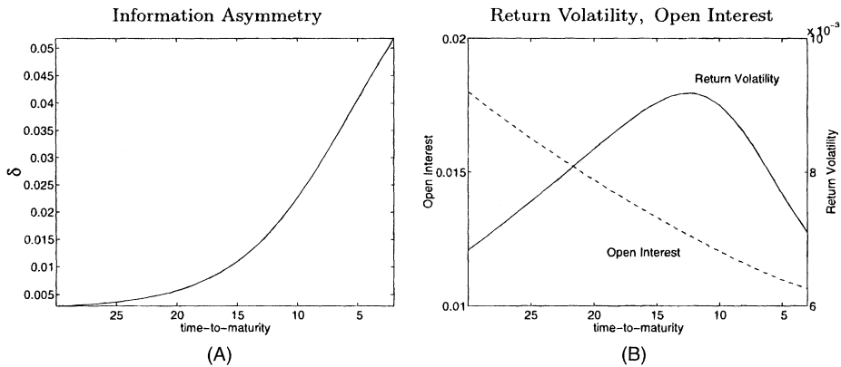
Figure 3. Time-to-maturity patterns of information asymmetry, futures return volatility and open interest. The figures plot the time-to-maturity patterns of (A) information asymmetry, \delta , and (B) the return volatility and open interest of the k -th contract. The parameters are set at the following values: \kappa_{Dq} = 0.5 , \sigma_D = 0.2 , \sigma_q = 0.025 , a_Z = 0.98 , \sigma_Z = 0.025 , a_{Y_1} = 0.97 , \sigma_{Y_1} = 0.075 , a_{Y_2} = 0.8 , \sigma_{Y_2} = 0.05 .
