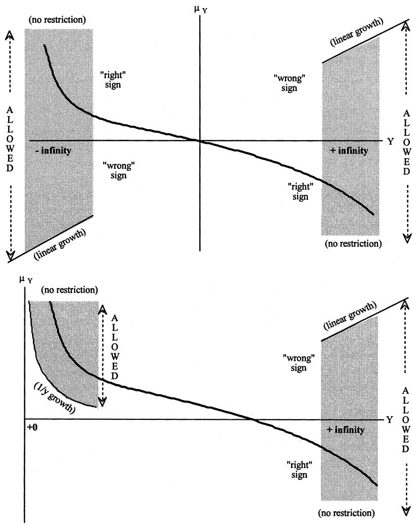
Figure A1. Growth conditions for the drift \mu_Y(Y;\theta) . This figure translates graphically the assumptions made in the Appendix regarding the shape of the function \mu_Y . The admissible shape of the function is substantially less restricted than under the standard growth conditions. In particular, I only restrict the growth of \mu_Y when it has the “wrong” sign (positive near +\infty , negative near -\infty ).
