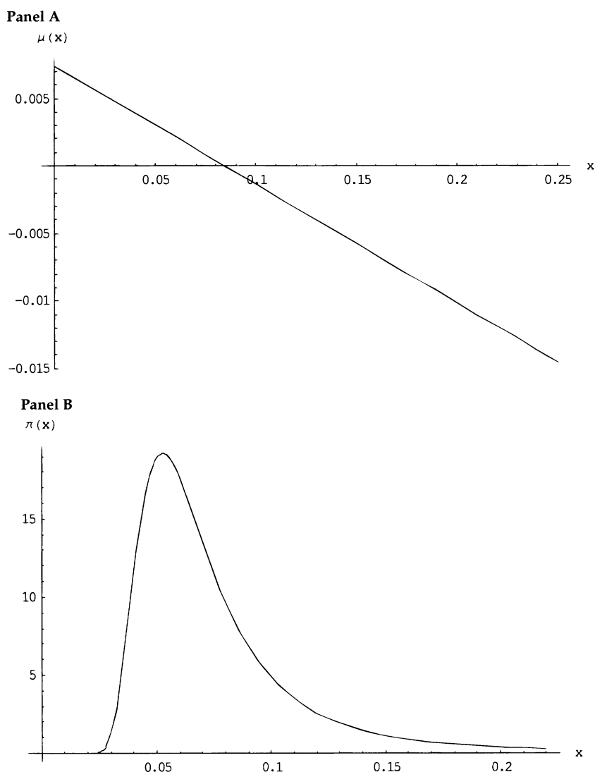
Figure 4. Conditional density approximations for the linear drift, CEV diffusion model.
