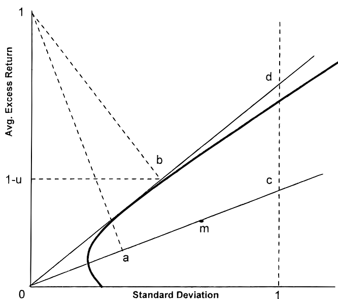
Figure 1. Sample mean standard deviation diagram. The point b is the point on the line Od that is closest to the point (0,1) and the point a is the point on the line Om that is closest to (0,1) .
