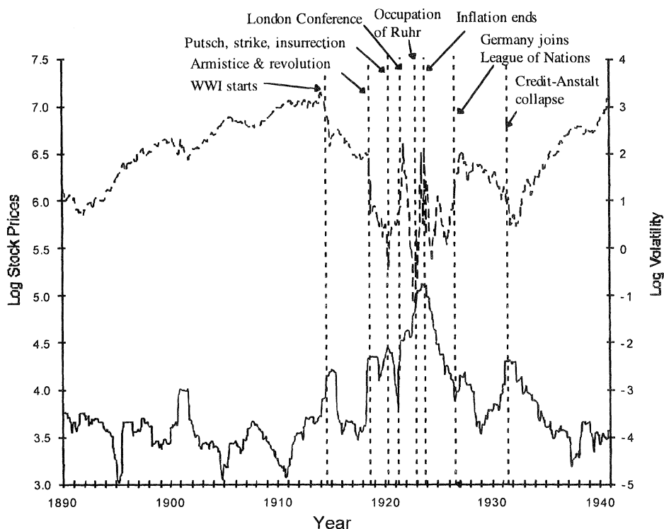
Figure 2. German political events, log of stock prices, and log volatility, monthly intervals, 1890–1940. The figure shows selected political events affecting Germany, the natural log of real, dividend-adjusted stock prices in month s (— — —), and the natural log of the twelve-month rolling standard deviation of returns in months s - 6 through s + 5 . Both series are shown at monthly intervals for January 1890 through December 1940. Data are from Gielen (1994).
