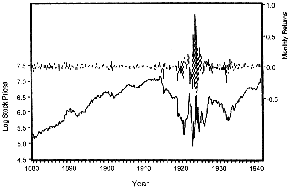
Figure 1. German stock prices and stock returns, monthly intervals, 1880–1940. The natural log of real, dividend-adjusted German stock prices (—) are shown on the left scale, and monthly returns (— — —) are shown on the right scale. Both series are shown at monthly intervals for January 1880 through December 1940. Data are from Gielen (1994).
