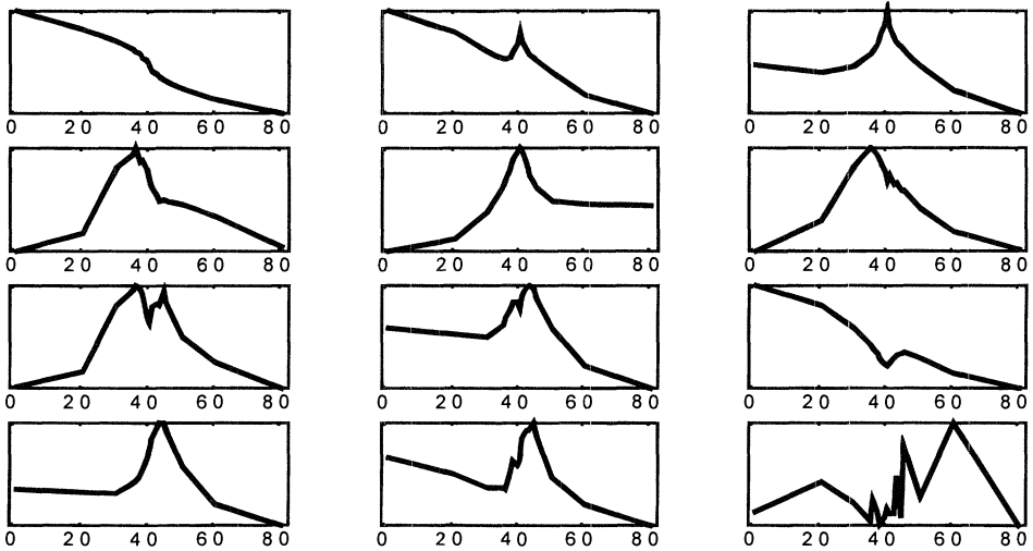
Figure 4. Twelve prominent sell indicators. FEVA plots representing the “structure” of the DJIA time series. We obtain a 100-cluster solution for the enhanced dataset ( 27774 \times 49 matrix) and select the twelve prominent FEVA sell indicators from the solution. Patterns represent the price path of the DJIA over the eighty days preceding the forecast. The vertical axis is the price and the horizontal axis represents the number of days used to construct the feature vector.
