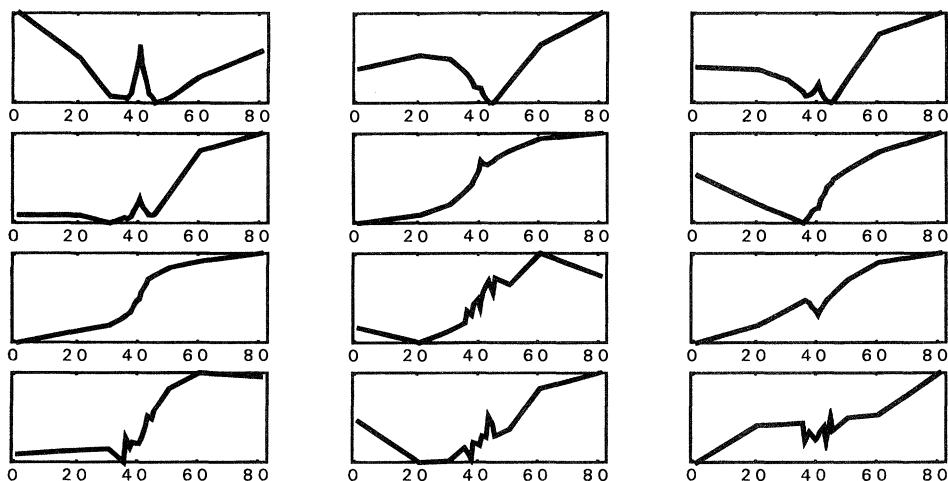
Figure 5. Twelve prominent buy indicators. FEVA plots representing the “structure” of the DJIA time series. We obtain a 100-cluster solution for the enhanced dataset ( 27774 \times 49 matrix) and select the twelve prominent FEVA buy indicators from the solution. Patterns represent the price path of the DJIA over the eighty days preceding the forecast. The vertical axis is the price and the horizontal axis represents the number of days used to construct the feature vector.
