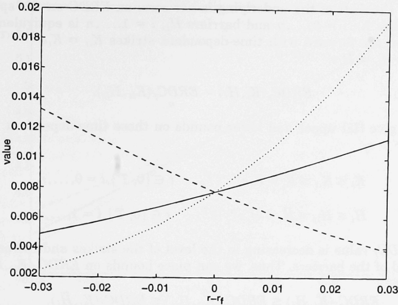
Figure 6. Synthesizing a double knockout call with cost of carry. Value of the upper (dashed line) and lower (dotted line) bound static hedges for a double knock-out call ( K = 100 , lower barrier 95, and upper barrier 105) compared with the analytical value (solid line). The foreign interest rate ( r_f ) is fixed at 4 percent and the domestic interest rate ( r ) varies from 1 percent to 7 percent. For r < r_f the lower bound is the upper bound and vice versa.
