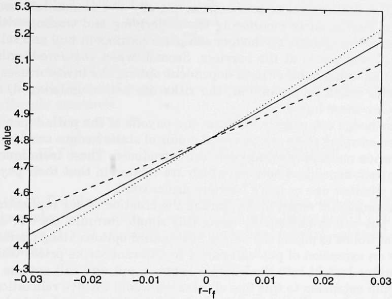
Figure 7. Synthesizing a roll-down call with cost of carry. Value of the upper (dashed line) and lower (dotted line) bound static hedges for a roll-down call ( K_0 = 100, K_1 = H_1 = 95, H_2 = 90 ) compared with the analytical value (dotted line). The foreign interest rate is fixed at 4 percent and the domestic interest rate varies between 1 percent and 7 percent. When the domestic rate is below the foreign rate, the lower bound becomes the upper bound and vice versa.
