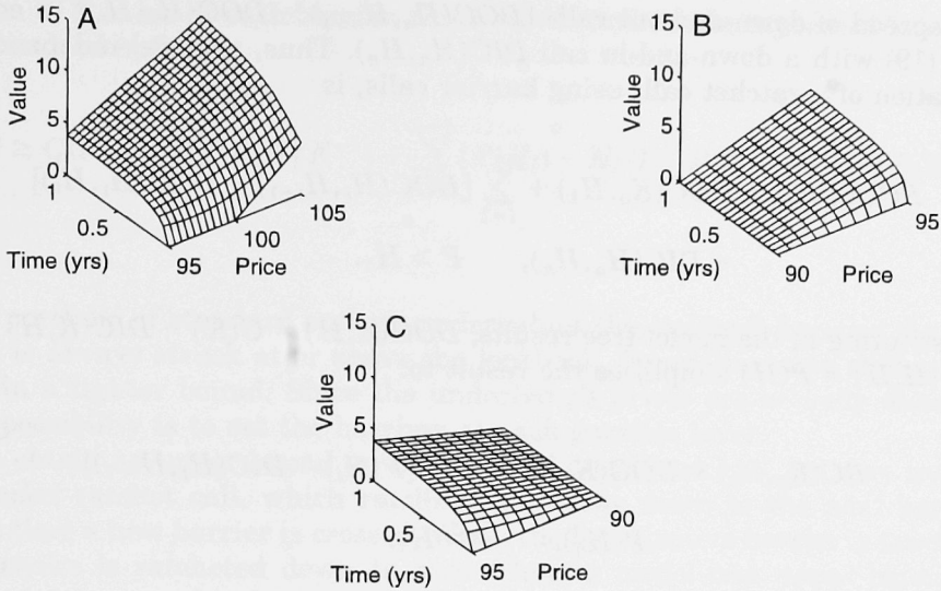
Figure 5. The two part static hedge for a roll-down call ( K_0 = 100 , K_1 = H_1 = 95 , H_2 = 90 ). Panel A shows the replicating portfolio when the price is above the first barrier, 95. Panel B shows the replicating portfolio after the barrier 95 has been hit. The two portfolios are identical along the barrier of 95, and the second is worth zero along the lower barrier 90. Panel C is a different perspective of Panel B, showing more clearly value of the portfolio at 95.
