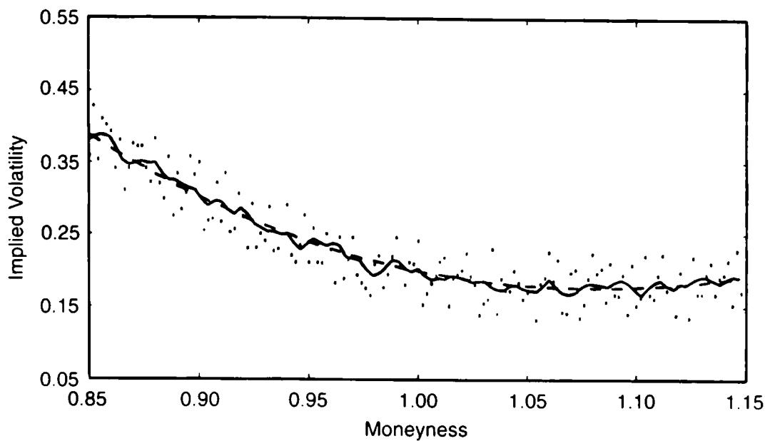
A: Kernel Regression with Undersmoothed Bandwidth
