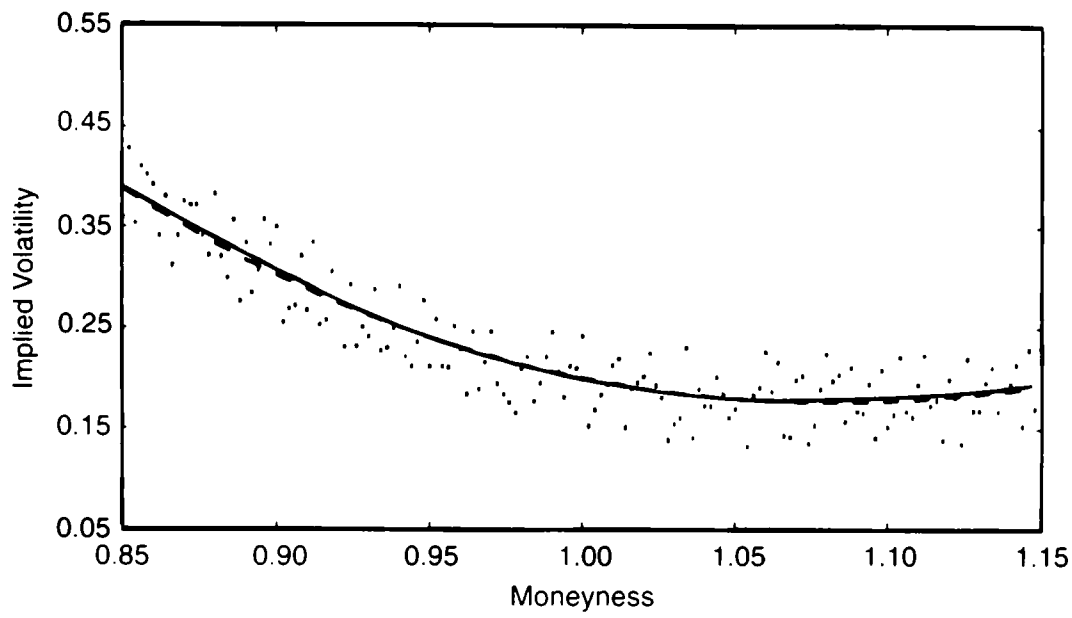
B: Kernel Regression with Optimal Bandwidth
