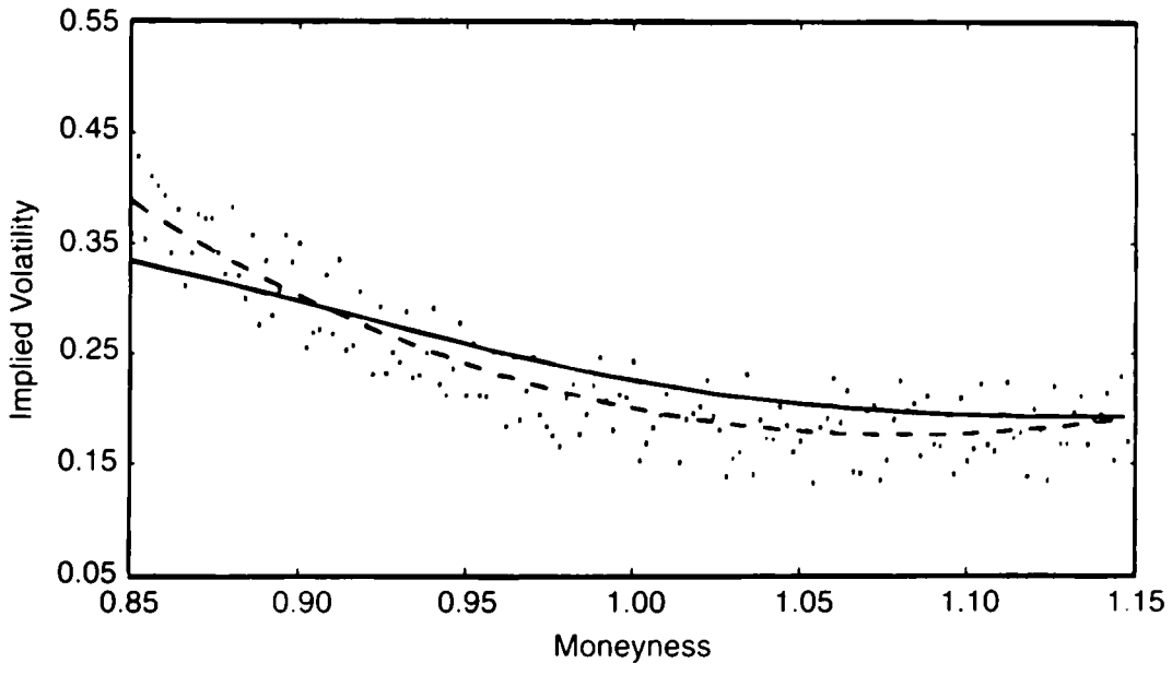
C: Kernel Regression with Oversmoothed Bandwidth
