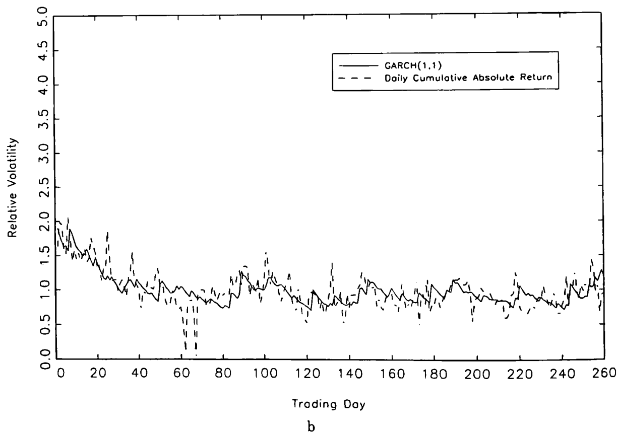
Figure 2. Daily GARCH(1,1) volatility forecasts versus ex post return variability mea- sures. The figures plot the conditional return standard deviation forecasts from an MA(1)- GARCH(1,1) model for the daily deutsche mark-dollar returns from October 1, 1992 through September 29, 1993, along with the corresponding realized absolute daily returns (Figure 2a) and the corresponding cumulative absolute five-minute returns (Figure 2b). All series have been normalized to average unity over the one-year sample.
