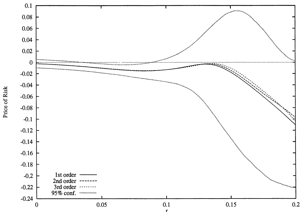
Figure 6. Estimated market price of interest rate risk. Estimates of first, second, and third order approximations to the market price of interest rate risk, \lambda(r) , are shown, calculated from daily excess returns on six month Treasury Bills, January 1965 to July 1995. Pointwise 95 percent confidence bands (for the first order approximation) are calculated using 10,000 iterations of the Künsch (1989) block bootstrap algorithm.
