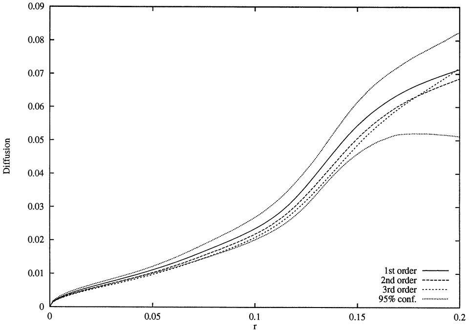
Figure 7. Constrained estimate of short rate diffusion. Estimates of first, second, and third order approximations to the diffusion, \sigma(r) , are shown, calculated using daily data, January 1965 to July 1995. All estimates are constrained to be zero at r = 0 . Pointwise 95 percent confidence bands (for the first order approximation) are calculated using 10,000 iterations of the Künsch (1989) block bootstrap algorithm.
