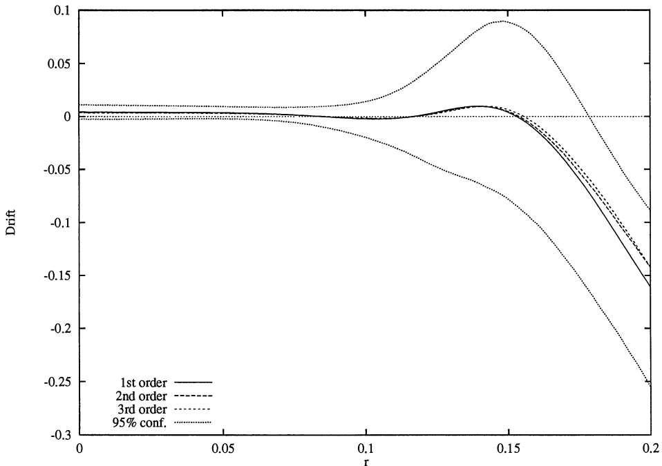
Figure 4. Estimated drift of short rate process. Estimates of first, second, and third order approximations to the drift, \mu(r) , are shown, calculated using daily data, January 1965 to July 1995. Pointwise 95 percent confidence bands (for the first order approximation) are calculated using 10,000 iterations of the Künsch (1989) block bootstrap algorithm.
