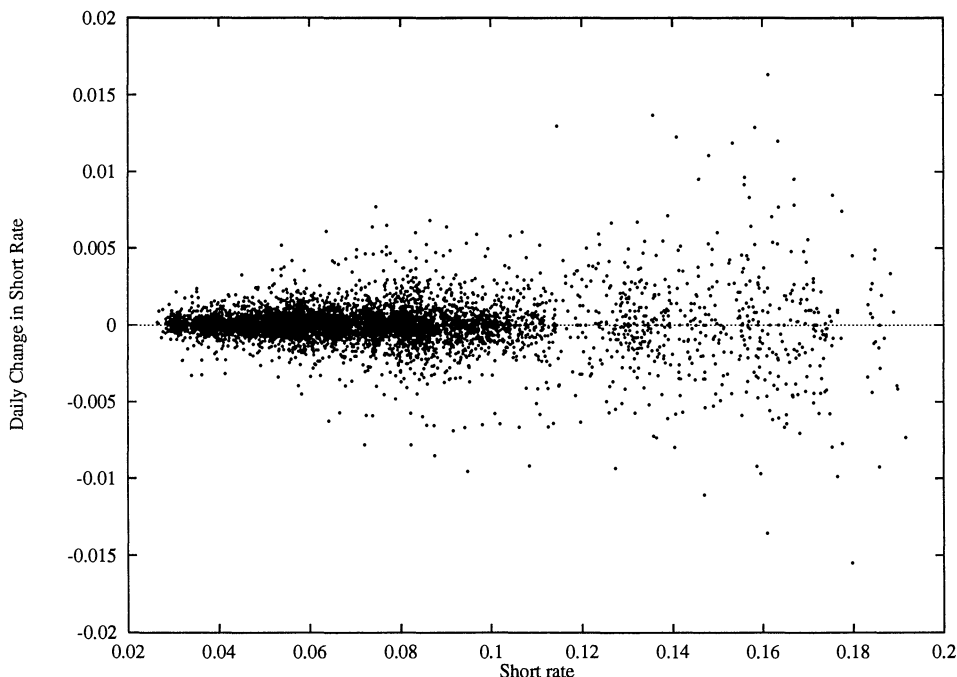
Figure 2. Daily interest rate changes, January 1965 to July 1995. Daily changes in the three-month Treasury Bill yield plotted against yield on preceding day.
