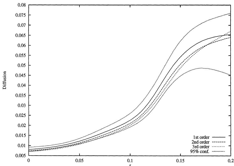
Figure 5. Estimated diffusion of short rate process. Estimates of first, second, and third order approximations to the diffusion, \sigma(r) , are shown, calculated using daily data, January 1965 to July 1995. Pointwise 95 percent confidence bands (for the first order approximation) are calculated using 10,000 iterations of the Künsch (1989) block bootstrap algorithm.
