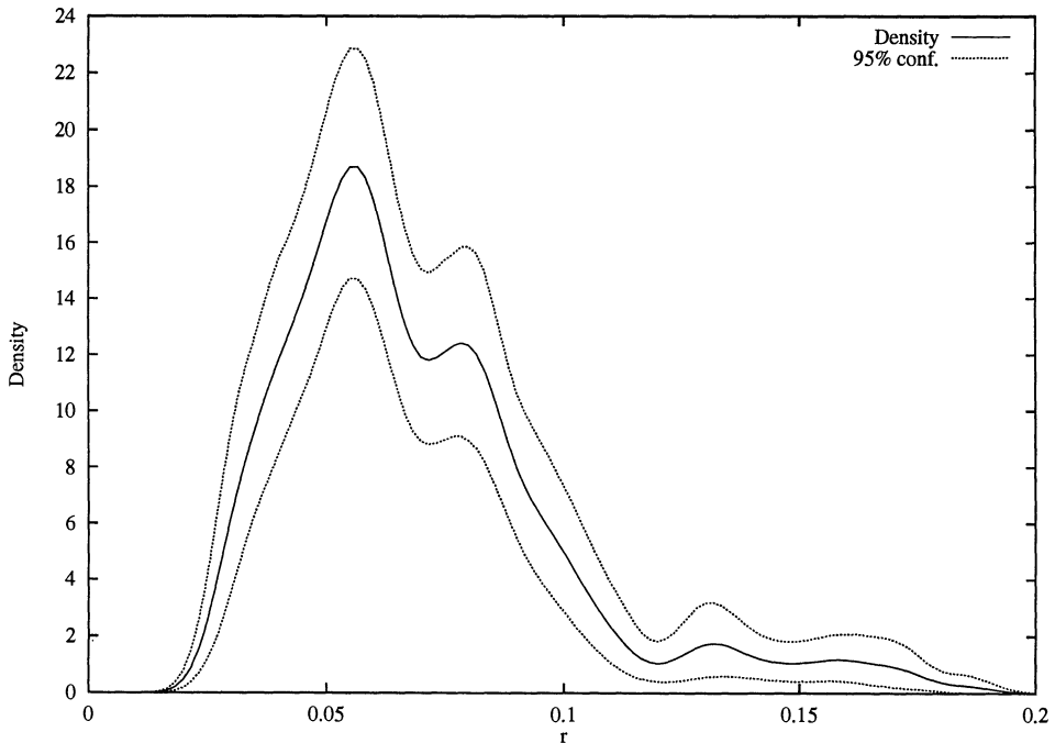
Figure 3. Estimated marginal density of short rate. Estimated marginal density of the three-month Treasury Bill yield, calculated using daily data, January 1965 to July 1995. Pointwise 95 percent confidence bands are calculated using 10,000 iterations of the Künsch (1989) block bootstrap algorithm.
