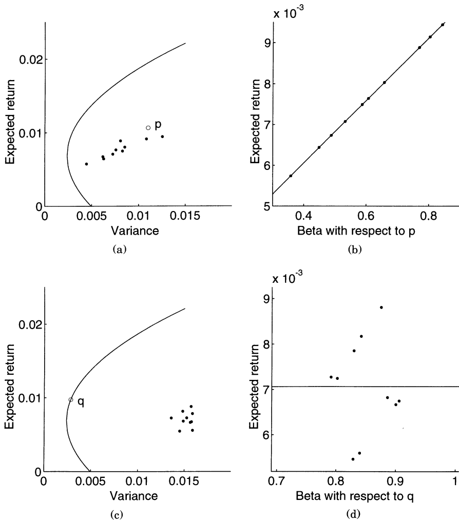
Figure 1. Examples of mean-beta relations for different mean-variance locations of the index portfolio. Figure 1a plots ten assets ( solid dots ), their minimum-variance boundary, and a portfolio p of those ten assets ( circle ). Figure 1b plots the expected returns and betas of those assets with respect to portfolio p as well as the OLS regression line through those points. Figures 1c and 1d display a similar case, except that the ten assets are a “repackaging” of those in the first case. The points in Figure 1b do not lie exactly on the regression line, and portfolio q in Figure 1c does not lie exactly on the minimum-variance boundary.
