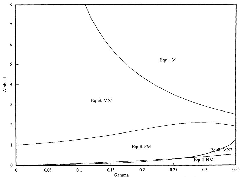
Figure 2. Existence conditions for the seasoned equity offering (SO) equilibria. This figure plots the regions of the parameter space (\alpha_I, \gamma) for which the various equilibria in the SO game exist. The three pure strategy equilibria are denoted by M, PM, and NM and are, respectively, the manipulation, partial manipulation, and nonmanipulation equilibria. The two mixed equilibria are denoted by MX1 and MX2. \alpha_I denotes the number of new shares allocated to the informed bidder when he participates in the SO. \gamma denotes the probability of observing an aggregate liquidity buy or sell order flow. The proportion of the offering allocated to uninformed bidders when both informed and uninformed bidders participate in the offering, 1/\beta , is kept fixed at 0.75.
