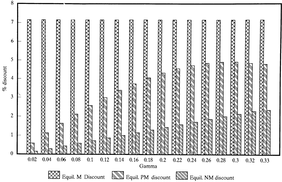
Figure 3. The seasoned equity offering (SO) equilibria issue discounts. The figure plots the issue discount as a function of \gamma for the three pure strategy equilibria. Equilibria M, PM, and NM are, respectively, the manipulation, partial manipulation, and nonmanipulation equilibria. \gamma is the probability of observing an aggregate liquidity buy or sell order flow. The discount is computed as a percentage of \Delta V , the difference between the high and low values of the asset. The proportion of the offering allocated to uninformed bidders when both informed and uninformed bidders participate in the offering, 1/\beta , is kept fixed at 0.75. The figure illustrates that the issue discount is unaffected by \gamma in the M equilibrium, while it is increasing in \gamma in the NM equilibrium. The issue discount is, however, nonmonotonic in \gamma in the PM equilibrium.
