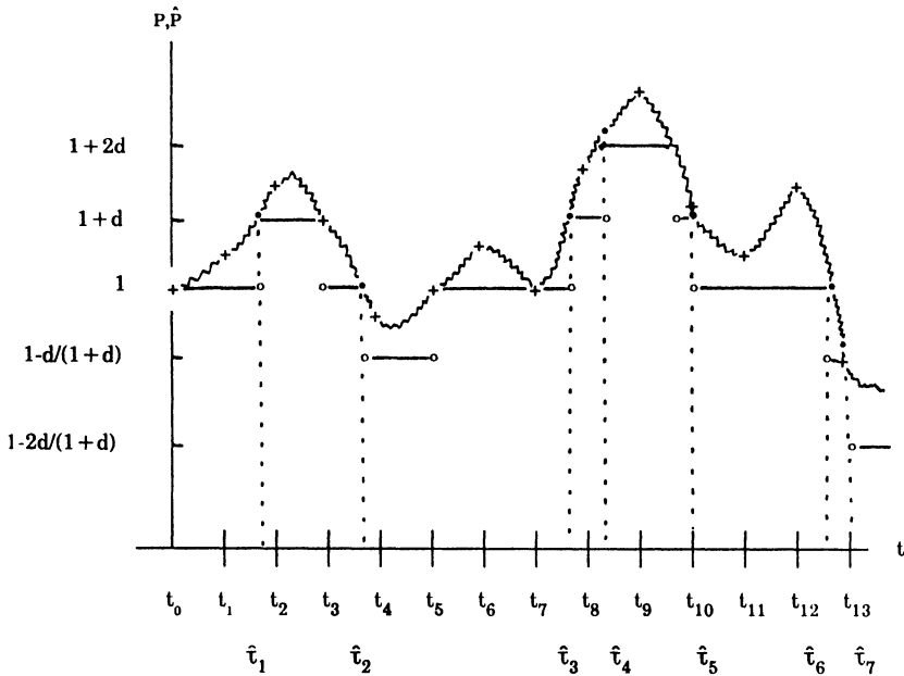
Figure 1. Stopping times of stock price changes. t_i , time at which price is generated; \hat{t}_i , estimated stopping time of price changes; \sim , true prices; —, observed prices; +, point at which true price is generated; •, point at which true price changes to the multiple of (1 + d) or (1 + d)^{-1} ; o, point of discontinuity.
