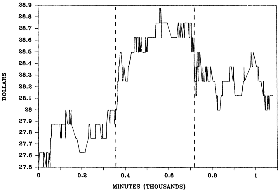
Figure 2. Transaction Stock Price of AMD (12/3/84-12/5/84).
