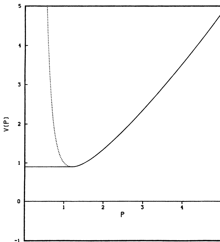
Figure 7. Value Functions for a Strategy of Switching between Two Time-Invariant Policies as P \geq P^* . (The functions shift up at a rate \gamma when P > P^* and at a rate r when P < P^* .)
