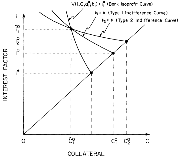
Figure 1. T2 Equilibria: IMRQ and \phi_1 = \phi_2
