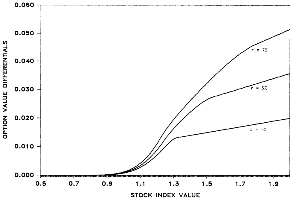
Figure 7. Option Value Differentials (Futures Minus Spot) – Stochastic Interest Rates. Exercise Price = 1, Volatility of Underlying Index Asset ( \sigma_1 ) = 0.25, Dividend Yield = 5%, Long-run Mean Interest Rate ( \mu ) = 10%, Volatility of Interest Rate ( \sigma_2 ) = 0.09, Option Maturity = 9 Months.
