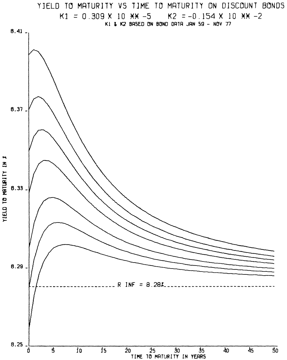
Figure 2. Yield to Maturity vs Time to Maturity on Discount Bonds K1 = 0.309 \times 10^{-5} K2 = -0.154 \times 10^{-2} K1 & K2 Based on Bond Data Jan 59-Nov 77
