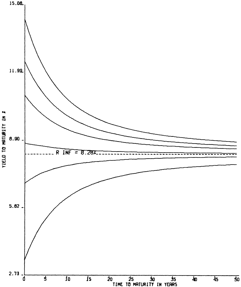
Figure 1. Yield to Maturity vs Time to Maturity on Discount Bonds
