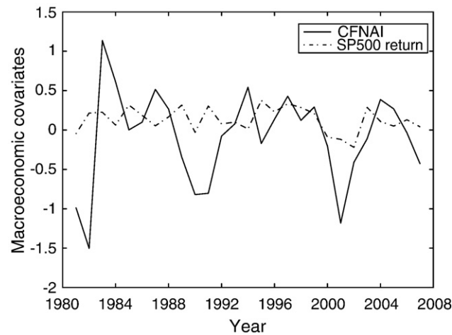
Fig. 1. History of the macroeconomic covariates CFNAI and S&P 500 return.
