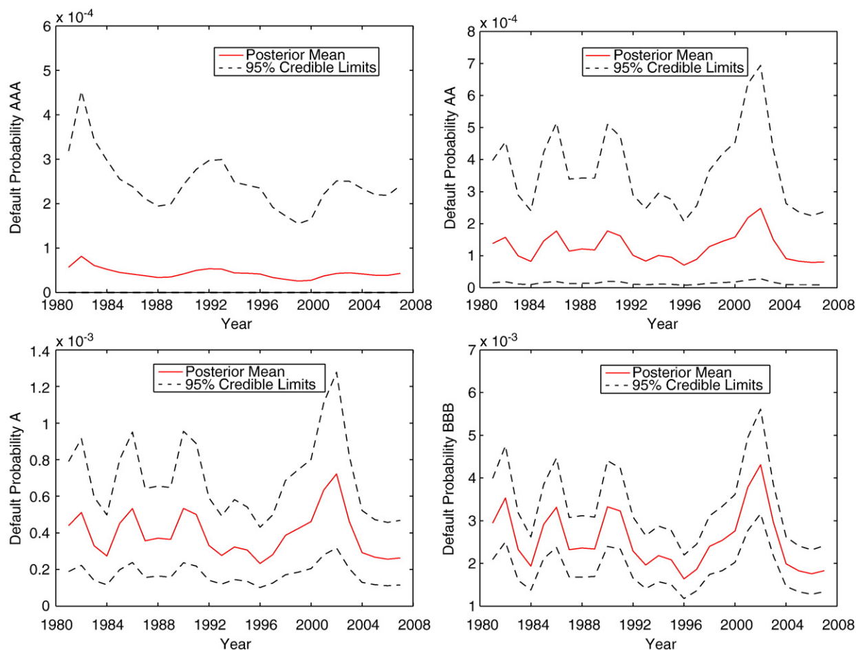
Fig. 3. Annual default probabilities (percentages) for investment grade ratings; posterior means with 95% credible intervals.
