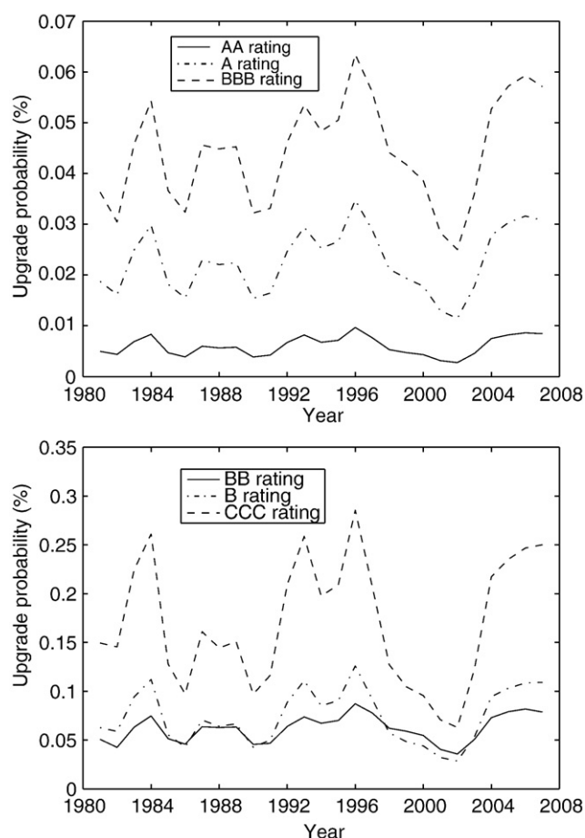
Fig. 5. Annual upgrade probabilities (percentages) for investment grade classes (upper graph) and speculative grade classes (lower graph).
