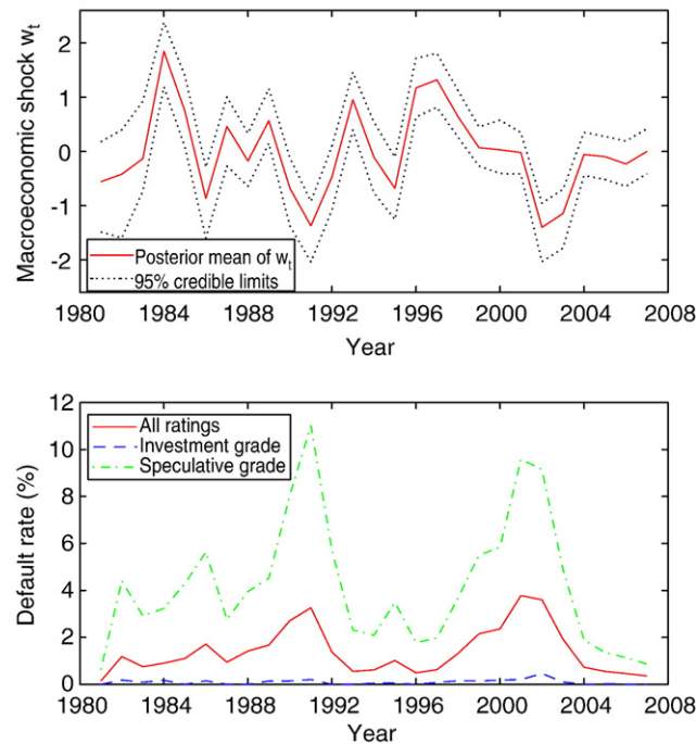
Fig. 2. Implied history of the macroeconomic shock w_t (upper graph) and historical default rates in percentages (lower graph).
