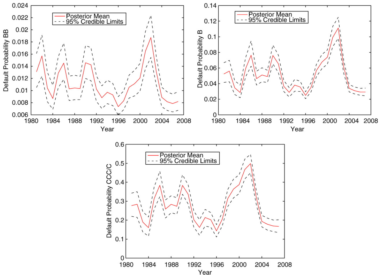
Fig. 4. Annual default probabilities (percentages) for speculative grade ratings; posterior means with 95% credible intervals.
