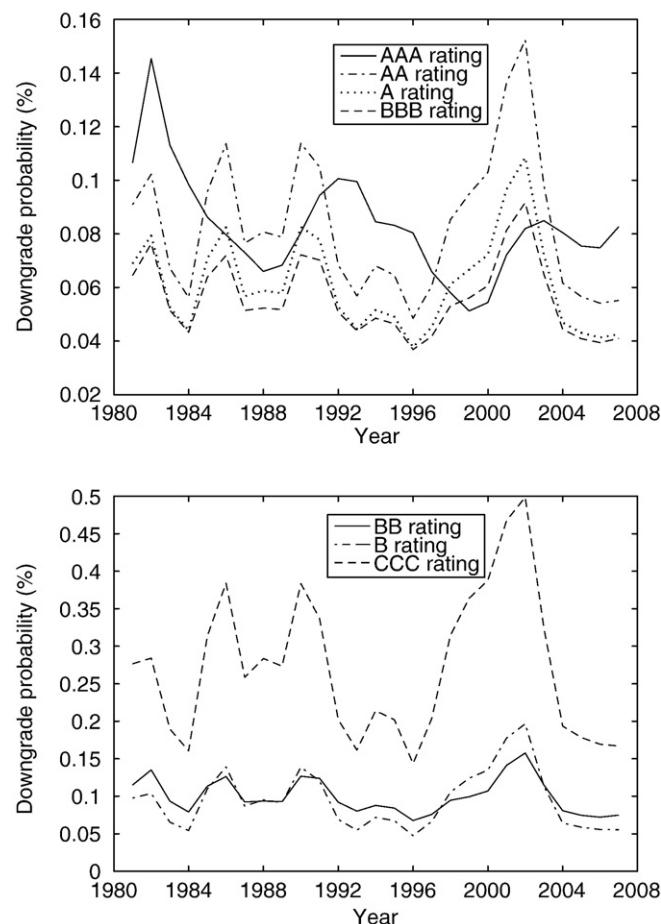
Fig. 6. Annual downgrade probabilities (percentages) for investment grade classes (upper graph) and speculative grade classes (lower graph).
