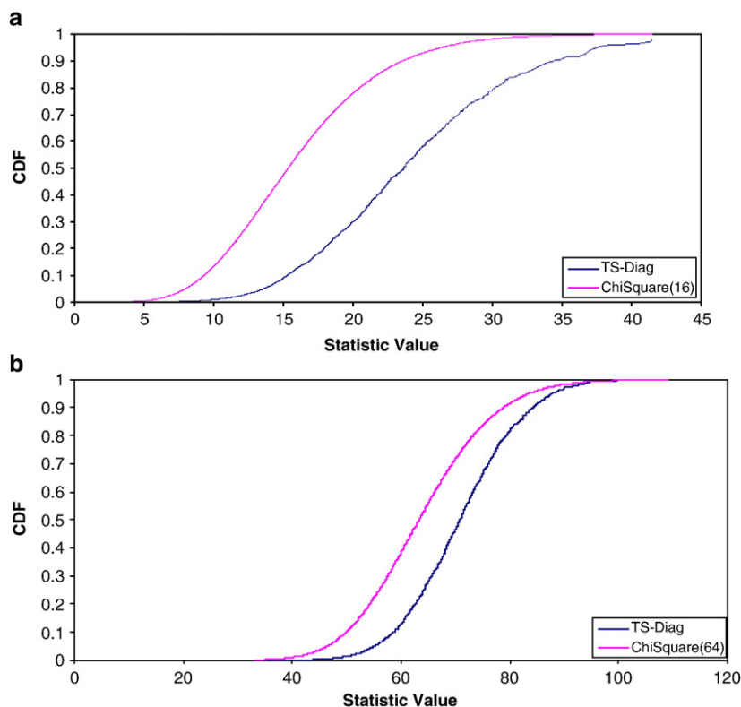
Fig. 1. a: TS-Diag Distribution with k=5 , T=2 , and N=2000 . b: TS-Diag Distribution with k=5 , T=5 , and N=2000 .
