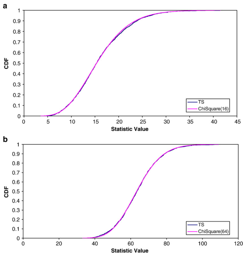
Fig. 3. a: TS_Sim Distribution with k=5 , T=2 , and N=2000 . b: TS_Sim Distribution with k=5 , T=5 , and N=2000 .
