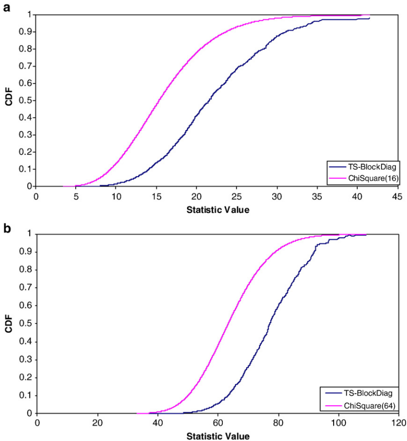
Fig. 2. a: TS_BlockDiag Distribution with k=5 , T=2 , and N=2000 . b: TS_BlockDiag Distribution with k=5 , T=5 , and N=2000 .
