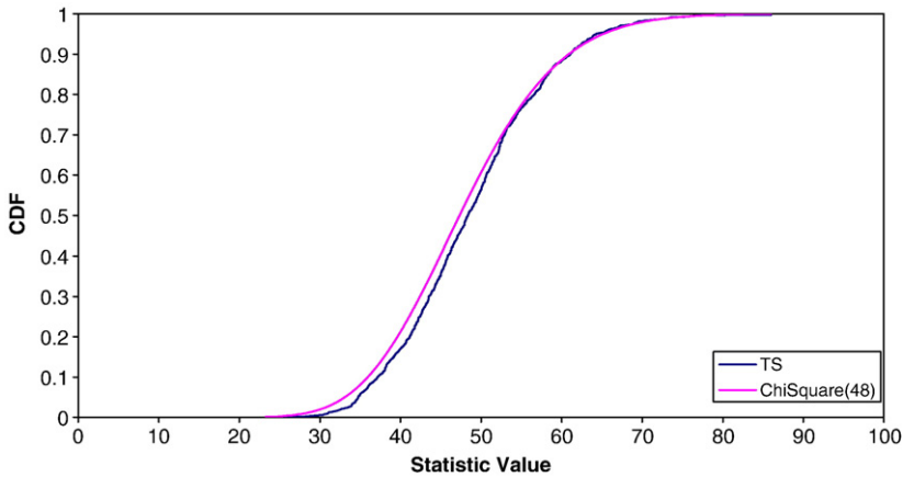
Fig. 4. TS_Sim Distribution with k=5 , T=3 , and N=1000 .
