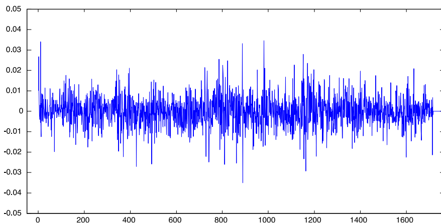
Fig. 1. Plot of the logarithmic USD/DEM exchange rate changes r_t , t = 1, \dots, 1716 ; January 2, 1988–December 30, 1994.
