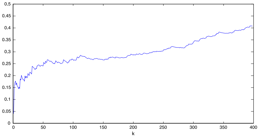
Fig. 2. Hill plot, \{(k, \hat{\xi}_{k,T}): 1 < k \leq 400\} , for the sample of exchange rate changes, T=1716 .
