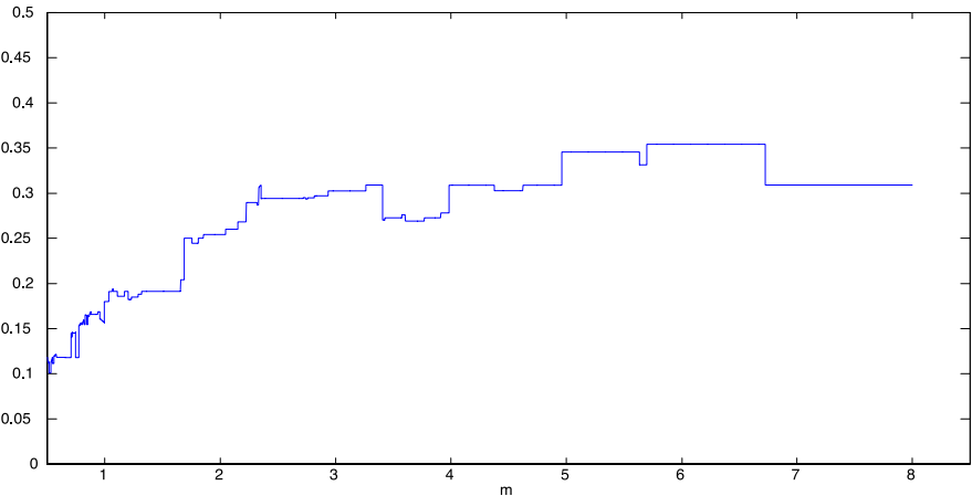
Fig. 4. MOT plot, \{(m, \hat{\xi}_{m,T}): 0 < m \leq 8\} , for the sample of exchange rate changes, T=1716 .
