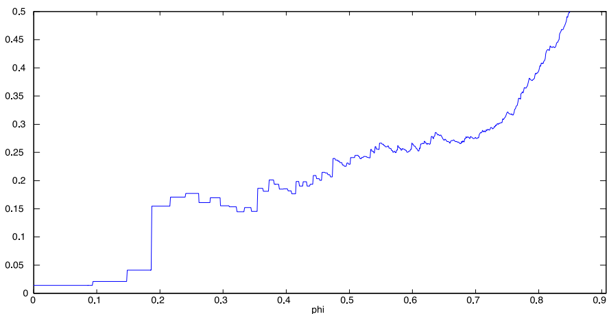
Fig. 3. Alternative Hill plot, \{(\varphi, \hat{\xi}_{\varphi,T}): 0 < \varphi \leq 0.9\} , for the sample of exchange rate changes, T=1716 .
