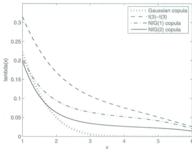
(b) Upper tail dependence
