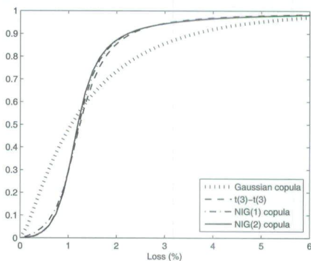
(a) Cumulative distribution function
