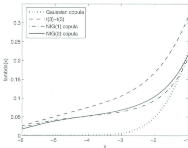
(a) Lower tail dependence
