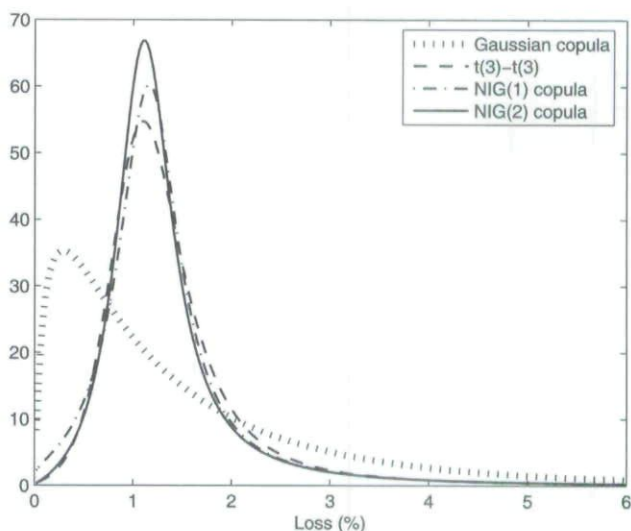
(b) Density function
