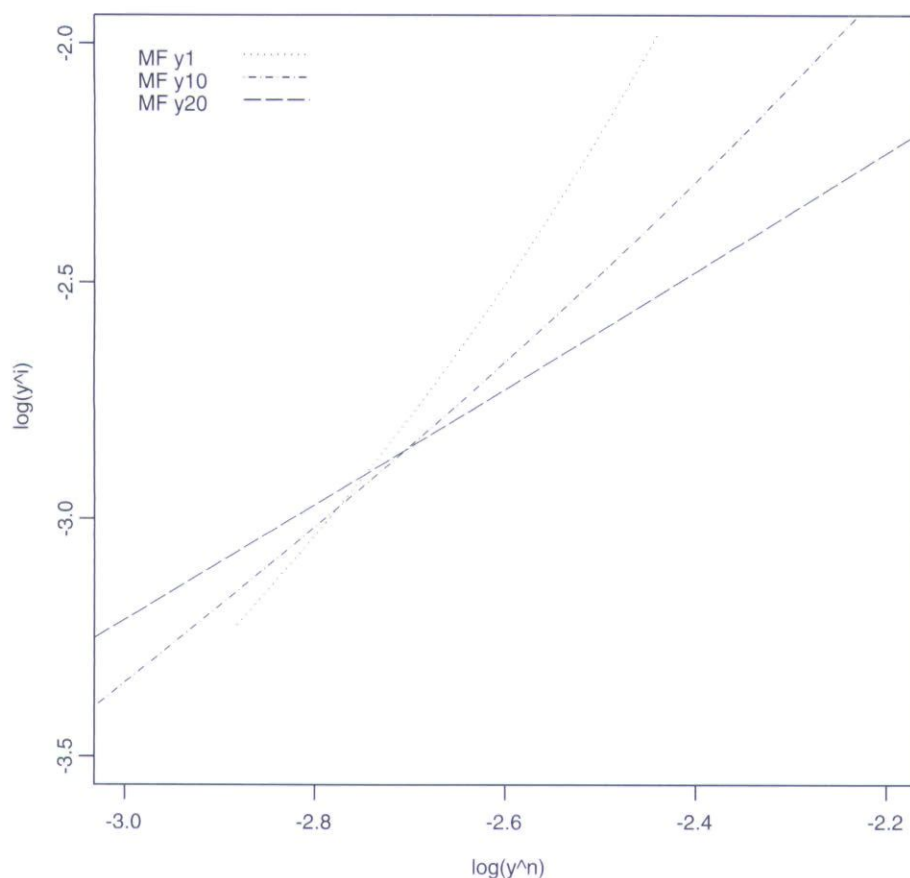
Graph of a Selection of Coterminous Forward Par Swap Rates \log(y_{T_i}^i) versus the Terminal Forward Rate \log(y_{T_i}^n) under the LIBOR MF model
