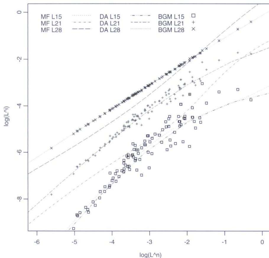
Plot of \log(L_{T_{15}}^i) versus \log(L_{T_{15}}^n) for Implied Caplet Volatilities of 50%
