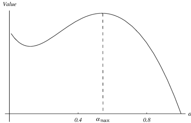
Fig. 6. The option value to carve out as function of the shares retained at the optimal threshold ( r=0.05 , \sigma_y=0.2 , \sigma_\varepsilon=0.7 , n=1 ).
