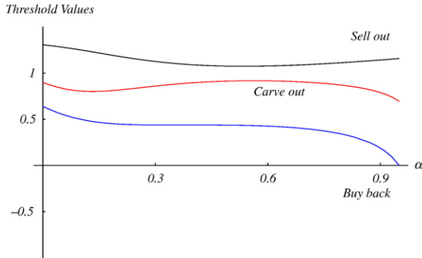
Fig. 2. Threshold values in terms of retained stake ( r=0.01, \sigma_y=0.2, \sigma_e=0.3, n=1 ).
