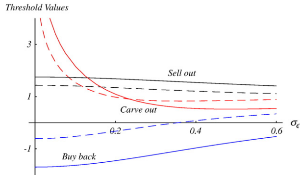
Fig. 4. Threshold values as a function of noise, for two values of uncertainty ( r=0.01 , \alpha=0.6 , n=1 ). Dashed line: \sigma_y=0.2 ; Normal line: \sigma_y=0.3 ).
