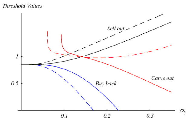
Fig. 3. Threshold values as a function of uncertainty, for two values of noise ( r=0.01 , \alpha=0.6 , n=1 ). Dashed line: \sigma_\varepsilon=0.1 ; Normal line: \sigma_\varepsilon=0.3 .
