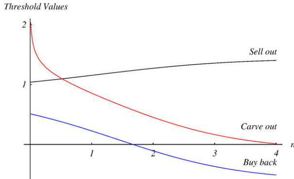
Fig. 5. Threshold value in terms of market informativeness ( r=0.01 , \sigma_y=0.2 , \alpha=0.6 , \sigma_e=0.3 ).
