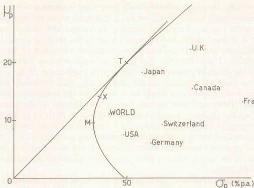
FIG. 1.—Geometry of the efficient set
