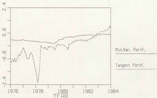
FIG. 3.—Weight of United States in optimal portfolio
