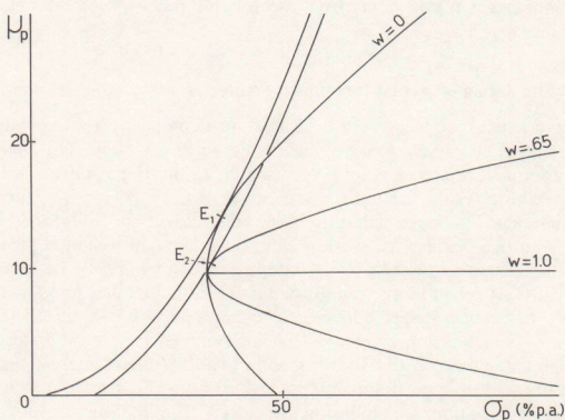
FIG. 2.—Efficient set and estimator choice
