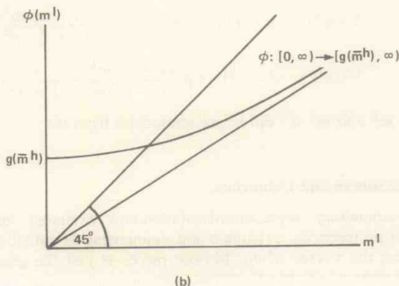
FIG. 1.—Existence of equilibrium
