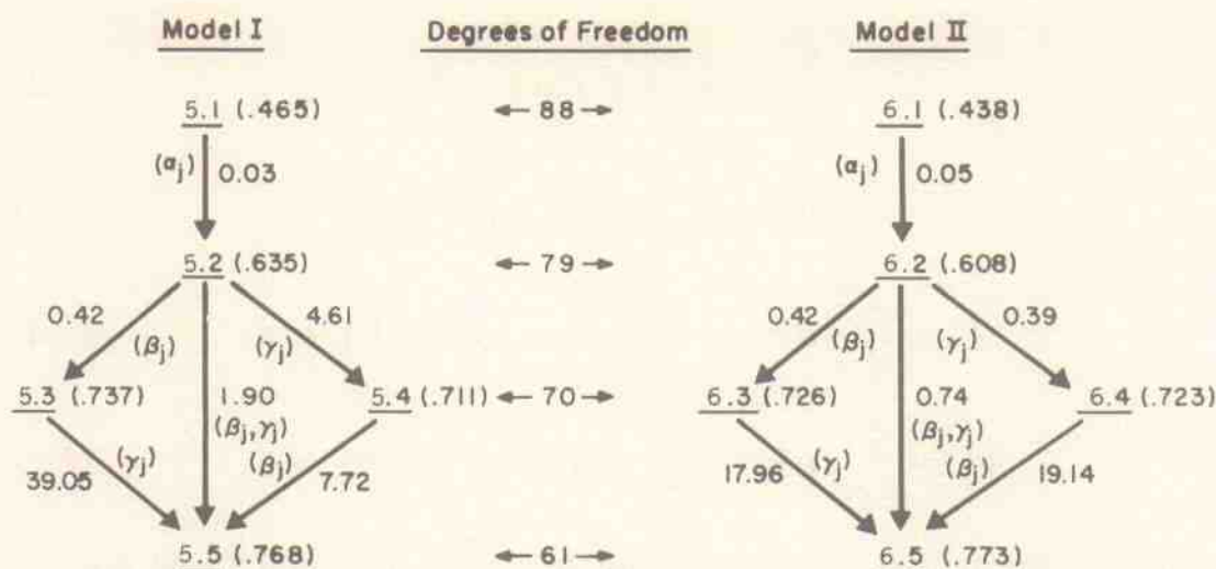
FIG. 2.— F -tests of nested specifications
