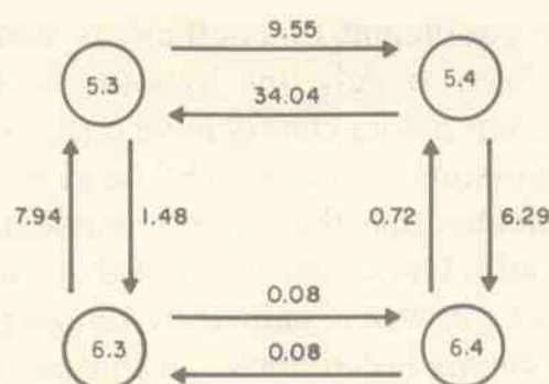
FIG. 3.—Nonnested specification tests
