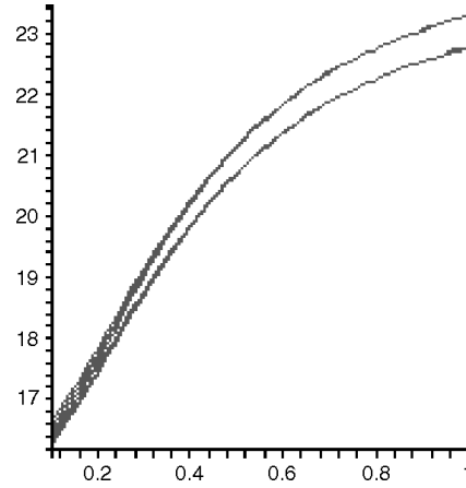
Figure 9. L_A(N_A, \overline{M}) - L_T(N_T, \overline{M}) = D2 ( \sigma_I on the horizontal axis).
