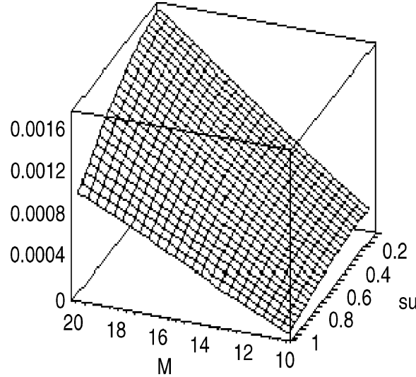
Figure 5. On the horizontal axes: M and su = \sigma_U , and on the vertical axis: Var(p^T) - Var(p^A) with a = 1 , \sigma_S = 0.8 , \sigma_\varepsilon = 0.5 , \sigma_I = 0.8 , \sigma_x = 0.8 , N = 20 , Z = 20 .
