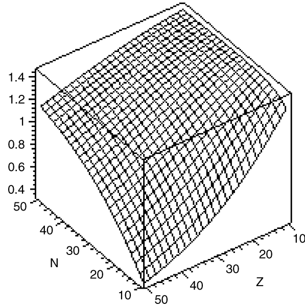
Figure 2. Adverse selection costs under anonymity. On the vertical axes: [[aVar(F|\Theta)]^{-1} - H] with a = 2, \sigma_\varepsilon^2 = 0.5, \sigma_I^2 = 0.5, \sigma_x^2 = 0.5, \sigma_S^2 = 0.5, M = 20 .
