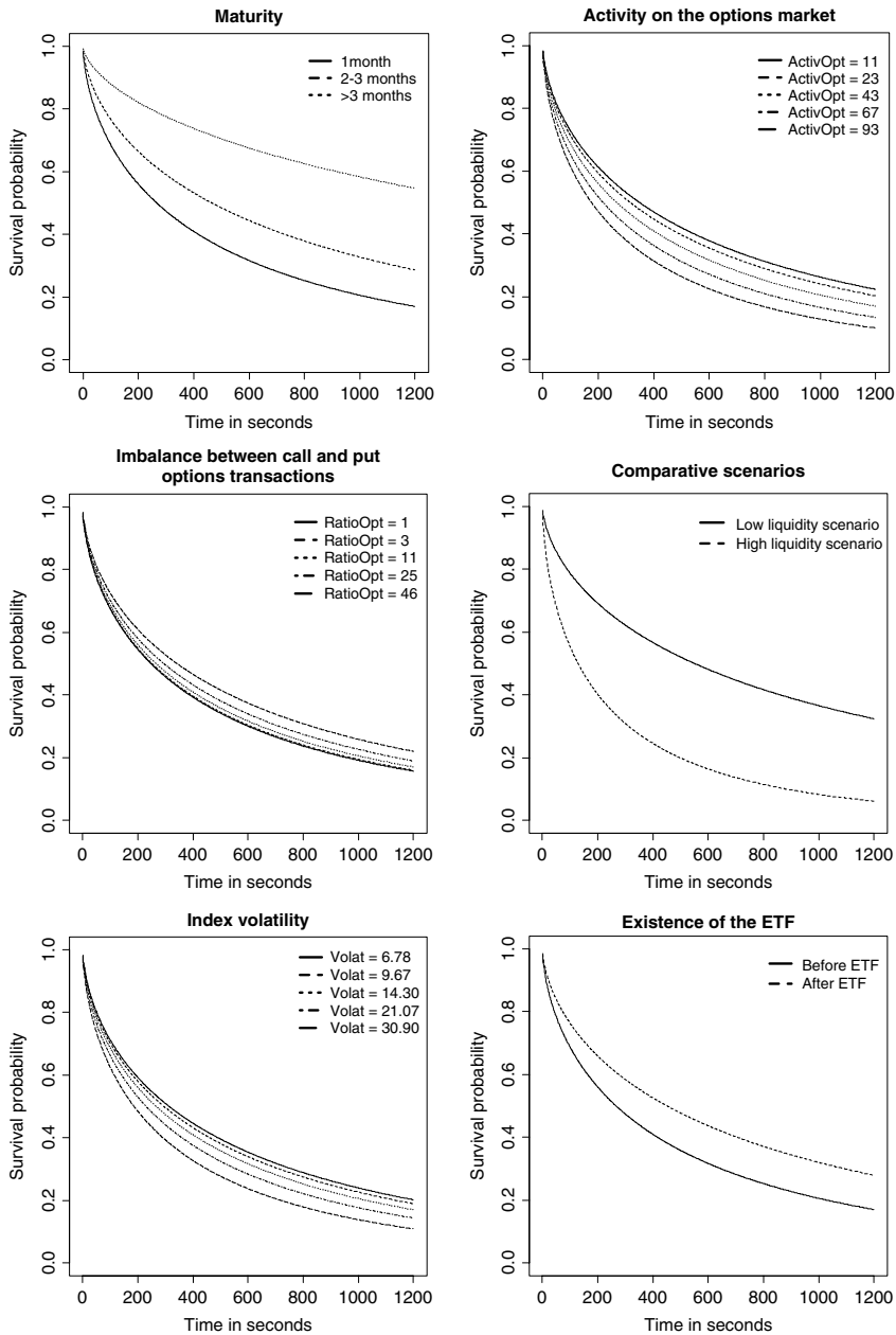
Figure 4. Sensitivity analysis
