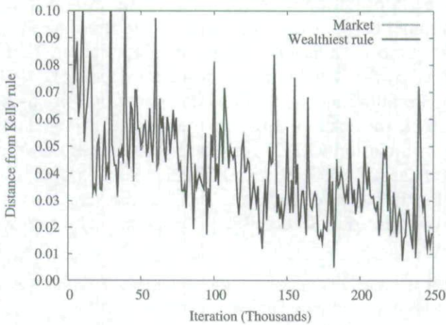
Figure 4. Euclidean distance between the Kelly rule and the wealthiest strategy resp. the market prices (which are virtually identical here) for price-dependent strategies.
