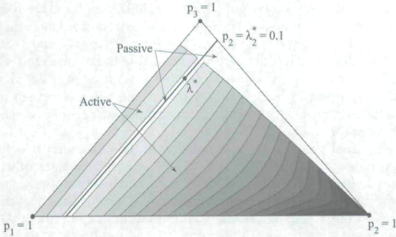
Figure 7. Contour plot of \delta(p) := \|\lambda^{LW}(p) - p\| for relative prices p = (p_1, p_2, p_3) in the unit simplex. \delta(p) is the Euclidean distance between the market portfolio p and the portfolio weights of strategy \lambda^{LW} in state 3. Darker areas represent larger values of \delta(p) , and white areas represent those prices for which \lambda^{LW} is in perfect agreement with the market portfolio, i.e., \delta(p) = 0 . Kelly prices and Kelly portfolio weights are given by \lambda^* = (0.2, 0.1, 0.7) .
