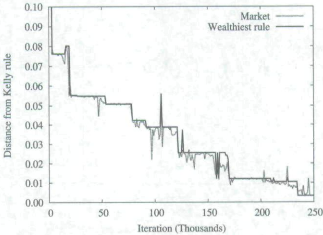
Figure 1. Euclidean distance between the market prices resp. the wealthiest strategy and the Kelly rule.
