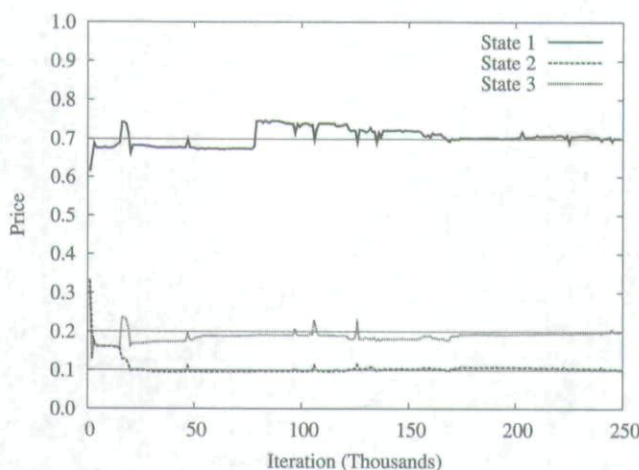
Figure 2. Relative price of Asset 1 by state and iteration. Horizontal lines correspond to the Kelly benchmark.
