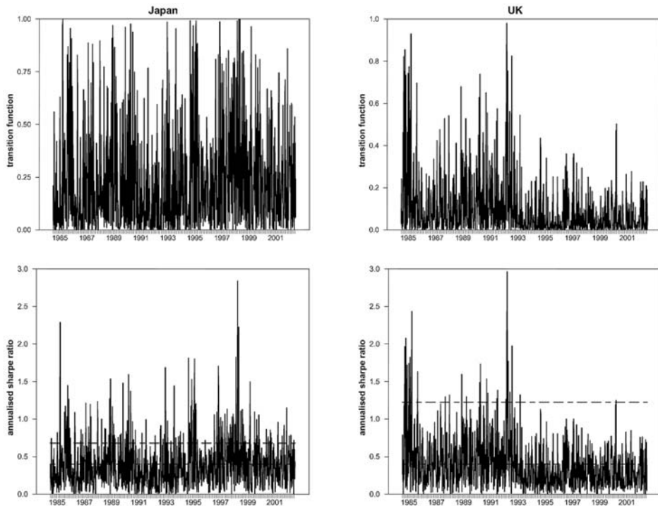
Figure 2. Sharpe ratios and estimated transition functions.
