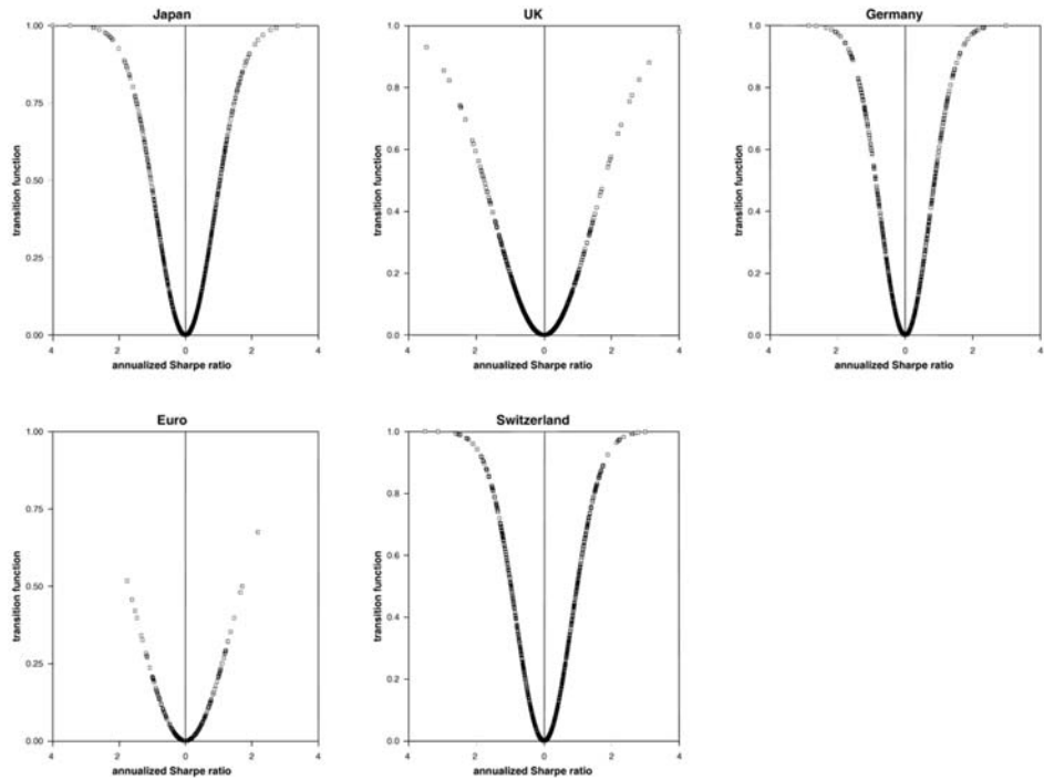
Figure 1. Estimated transition functions and Sharpe ratios.
