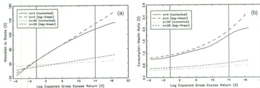
Figure 2. (a) Portfolio rule when \psi = 0.25 . (b) Consumption-wealth ratio when \psi = 0.25 .
