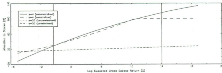
Figure 3. Unconstrained and constrained portfolio rule when \psi = 0.25 .
