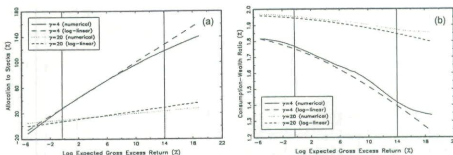
Figure 1. (a) Portfolio rule when \psi = 1.33 . (b) Consumption-wealth ratio when \psi = 1.33 .
