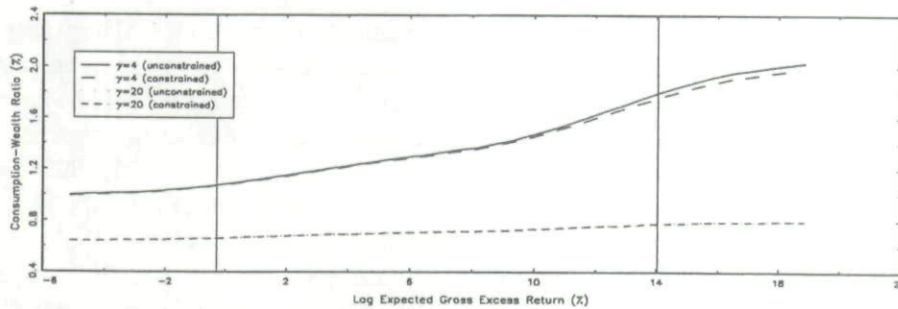
Figure 4. Unconstrained and constrained consumption-wealth ratio when \psi = 0.25 .
