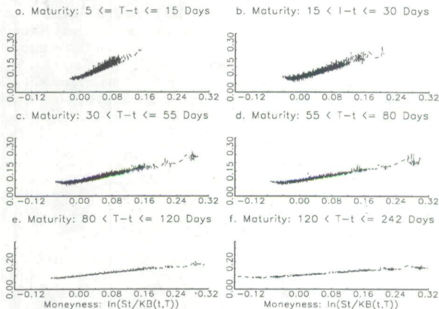
Figure 7. Implied Black-Scholes Volatility from Observed Option Prices.
