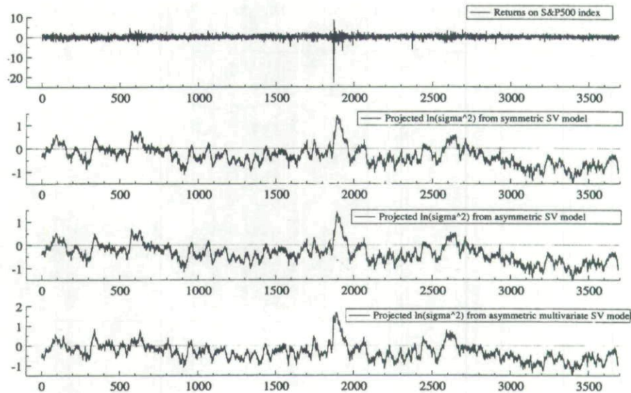
Figure 5. Filtered asset returns volatility for the SARMAV(1,0) and ASARMAV(1,0) models using reprojction. Daily observations 1980–1994.
