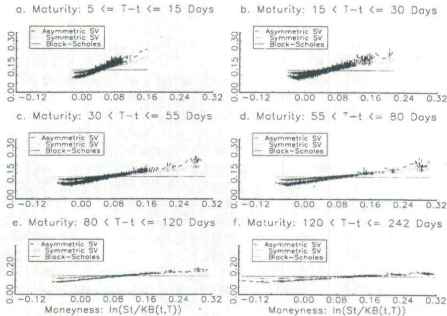
Figure 8. Implied Black-Scholes Volatility of Option Prices from Alternative Models based on Diversifiable Stochastic Volatility Risk.
