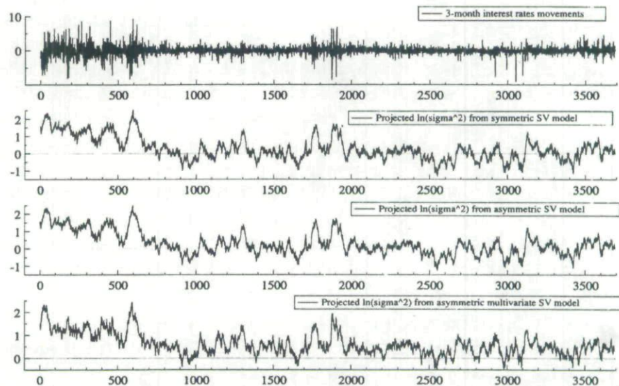
Figure 6. Filtered interest returns volatility for the SARMAV(1,0) and ASARMAV(1,0) models using reprojction. Daily observations 1980–1994.
